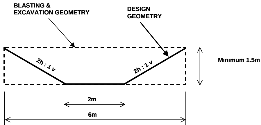
Figure 4. Design cross section for discharge channels through bedrock
