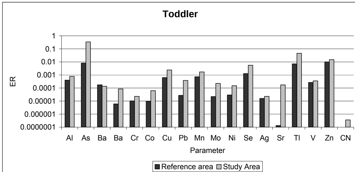
Figure 10 ERs for Toddler and Adult Based on Maximum Arsenic Concentrations
