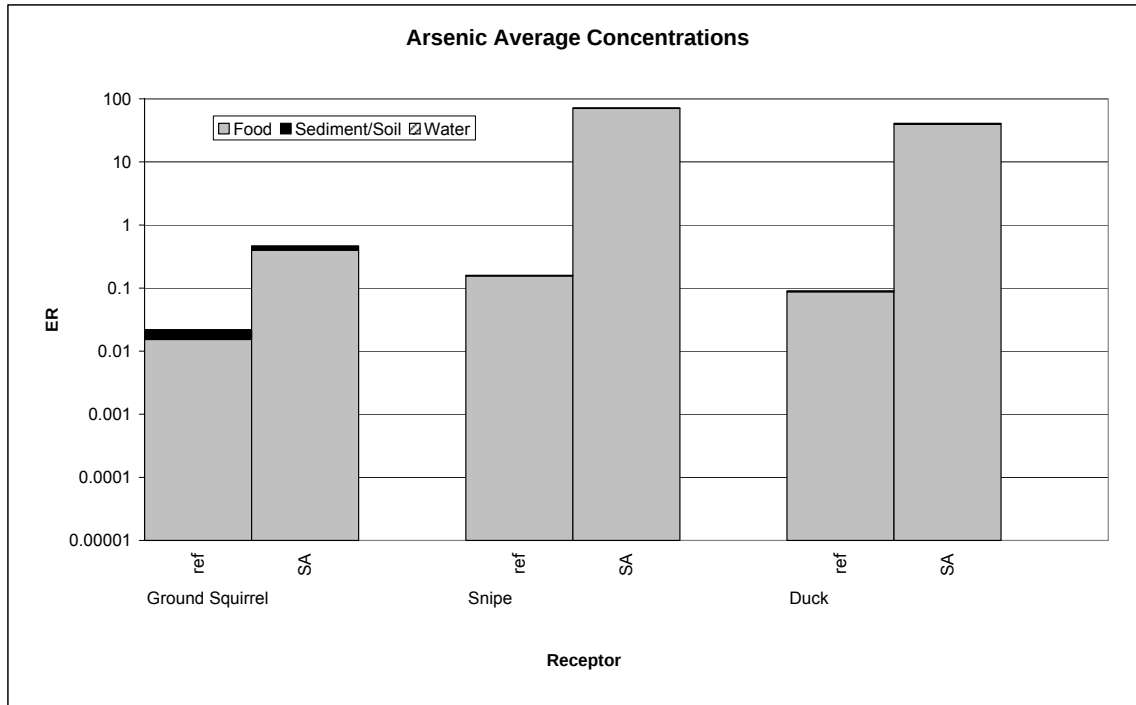
Figure 6 ERs for Arctic Ground Squirrel, Snipe and Long-Tailed Duck Based on Average Concentrations of Arsenic
