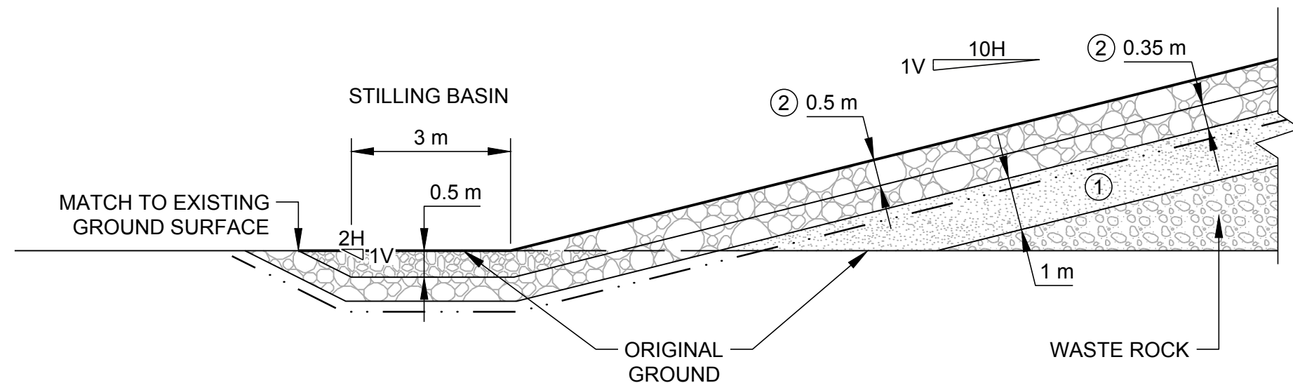
DRAINAGE CHUTE TYPICAL PROFILE N.T.S.
