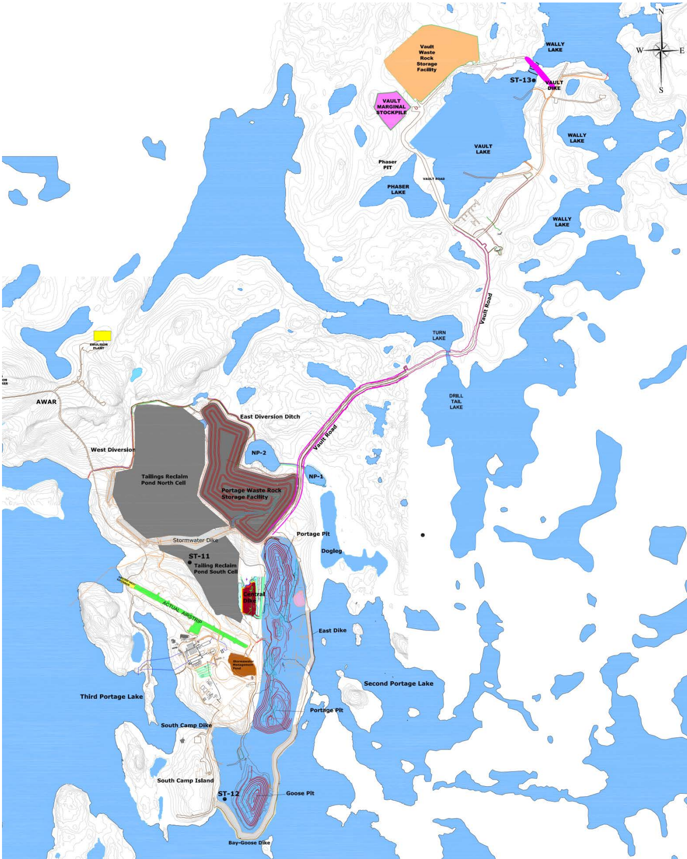
Figure 2-4: Post-Closure Phase
