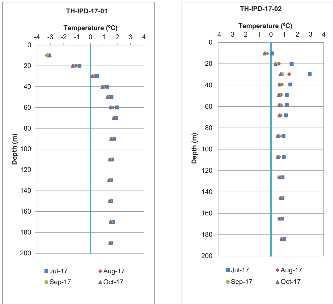
Figure 4-2 : Temperature Profiles - 2017 Hydrogeological Field Investigation
