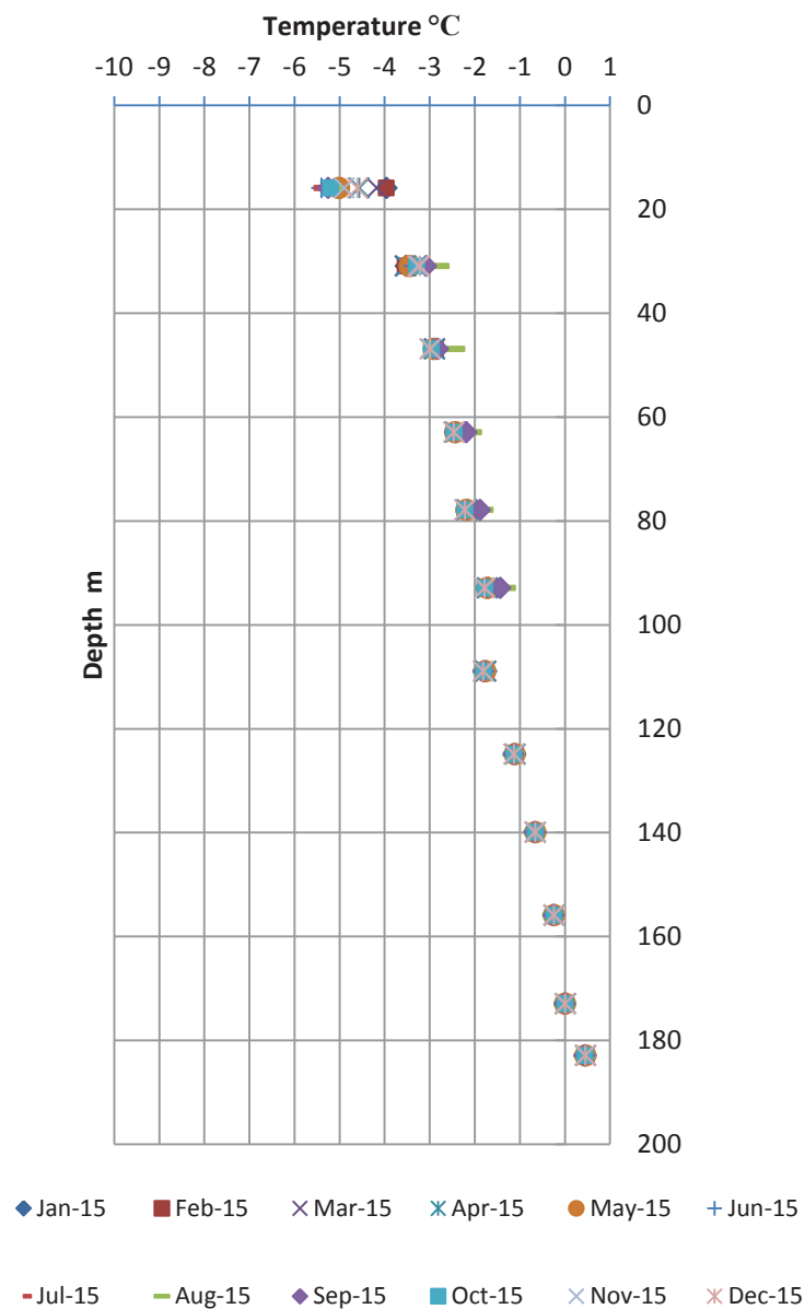
Figure 4-6: Ground Temperature Profile in 2015 at Borehole BG-GPIT17
