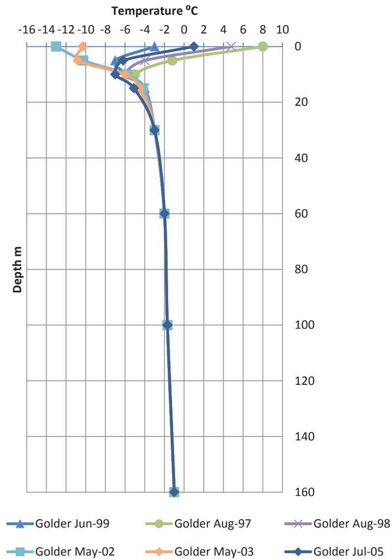
Figure 4-5: Ground Temperature Profile from 1997 to 2005 at Borehole TP97-196
