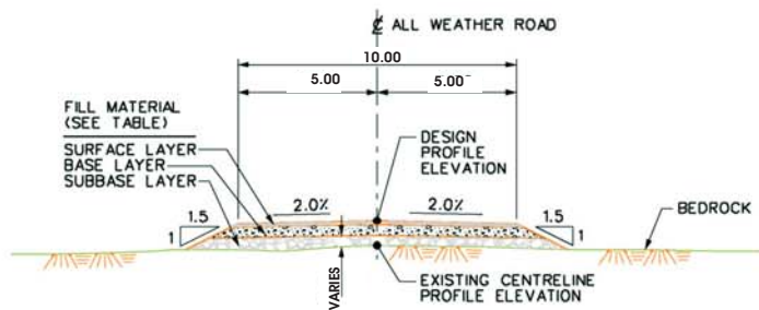
TYPICAL ALL WEATHER ROAD SECTION ON BEDROCK OR WELL-DRAINED GRANULAR SOILS
