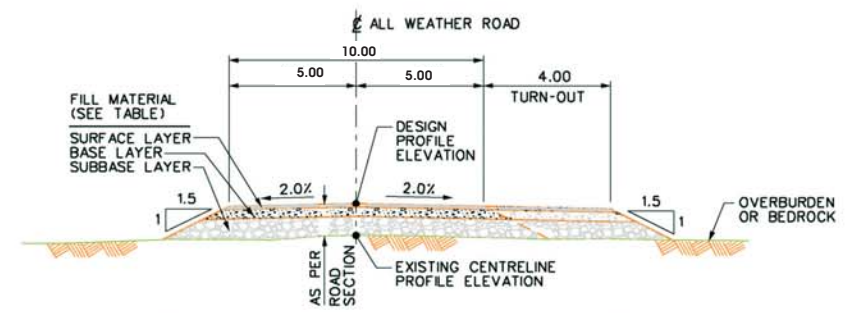
TYPICAL ALL WEATHER ROAD WITH TURN-OUT
