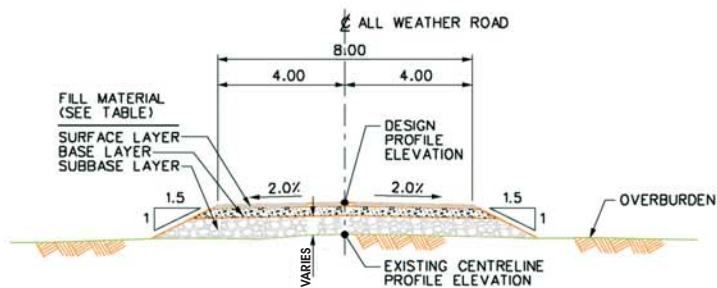
TYPICAL ALL WEATHER ROAD SECTION ON ICE-RICH SOILS
