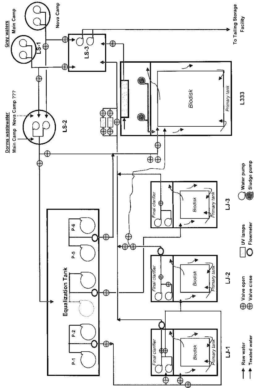
FIGURE 3.1: FLOWSHEET
