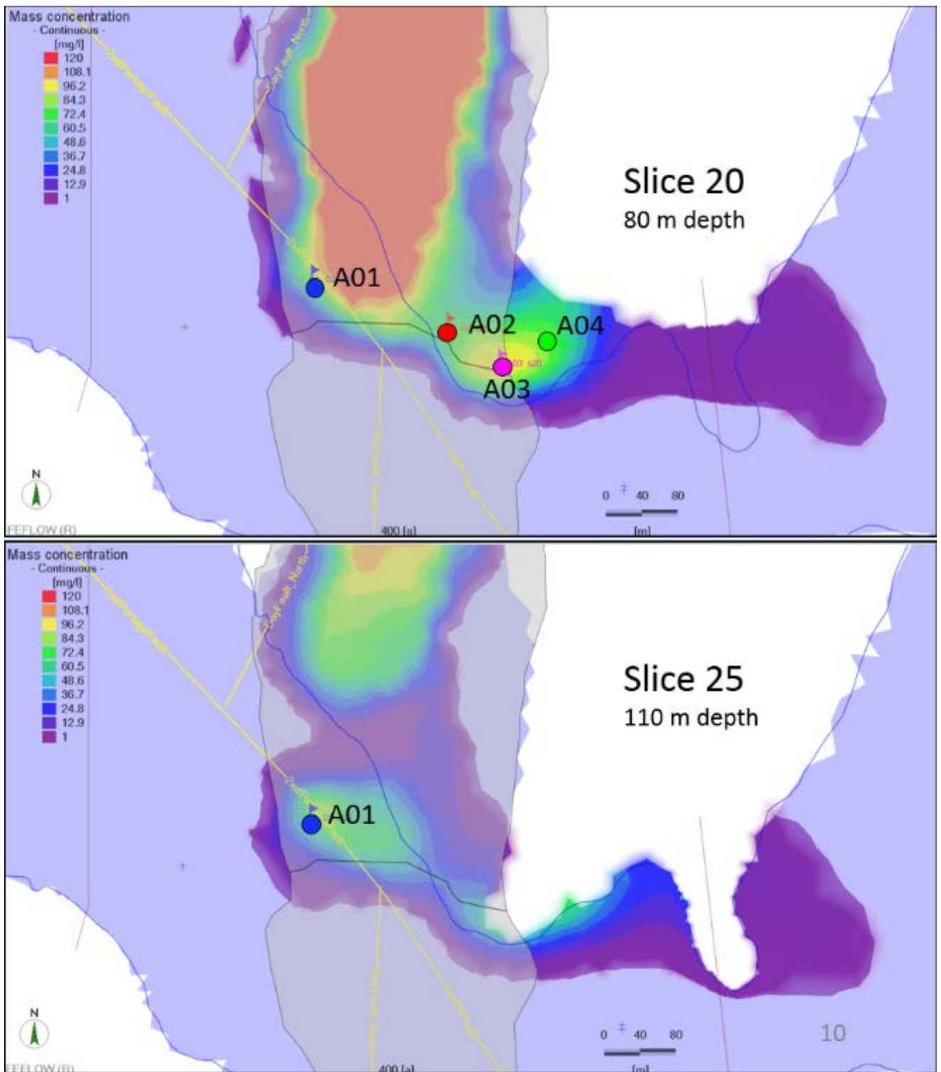
Figure 3: Predicted chloride plumes and Preliminary options for MWs to be installed at closure, Pit A, at t=400 years
