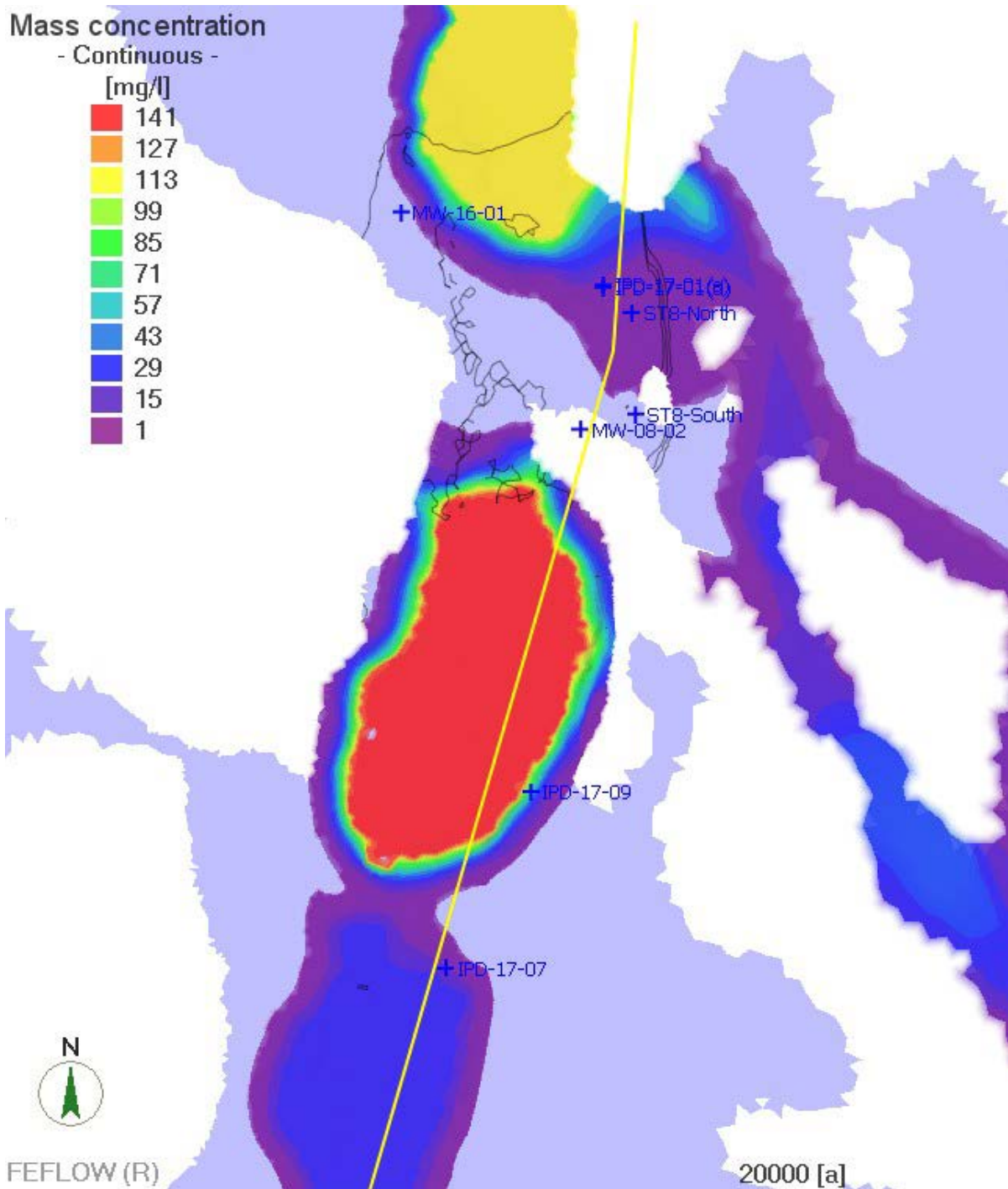
Figure 1: Location of the north-South cross-section with chloride plumes at t=20,000 years
