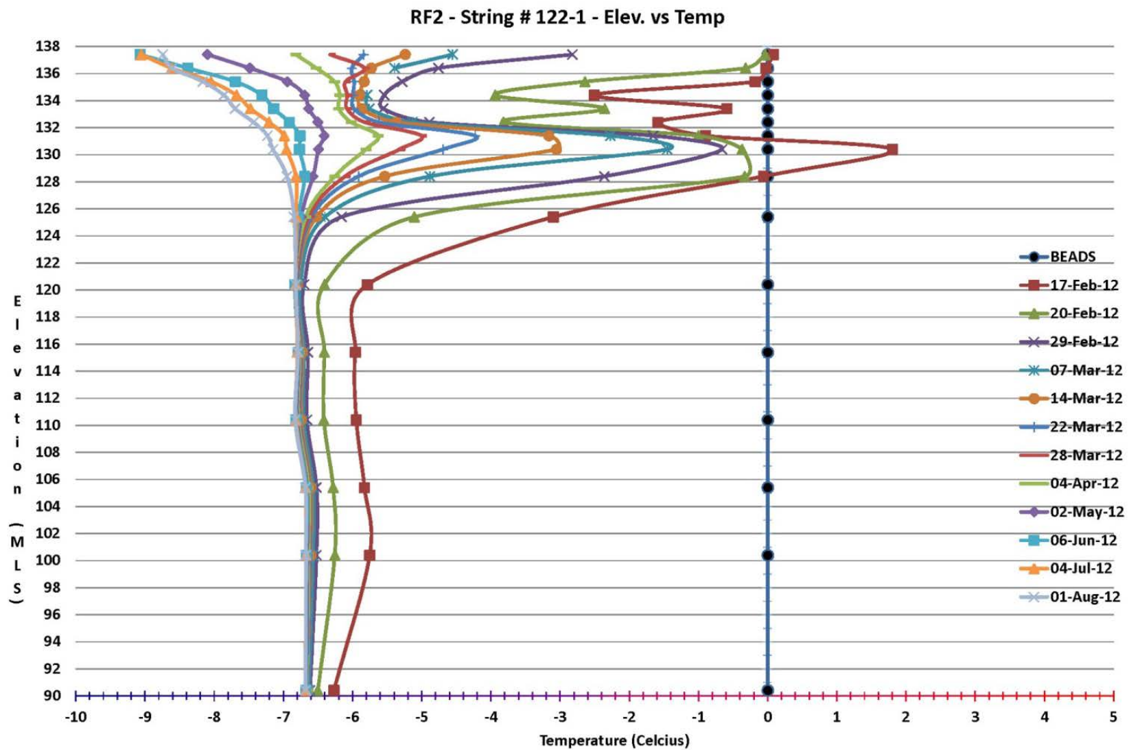
Figure 9: T122-1 Thermistor Results on RF2
