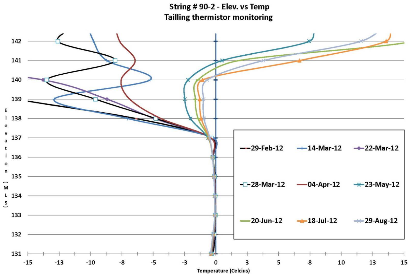
Figure 10: T90-2 Thermistor Results on TSF
