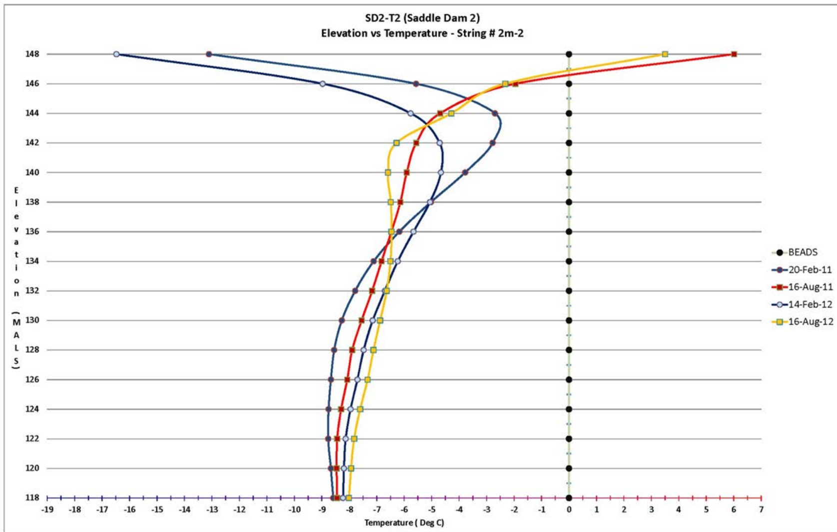
Figure 7: SD2-T2 Thermistor Results on Saddle Dam 2
