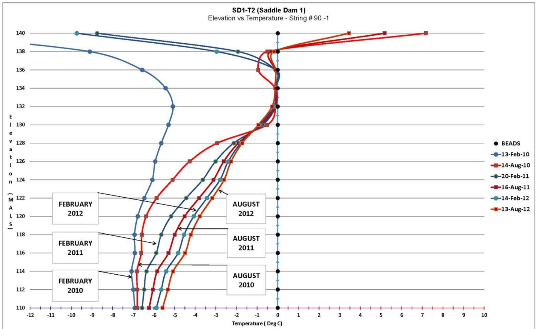
Figure 5: SD1-T2 Thermistor Results on Saddle Dam 1
