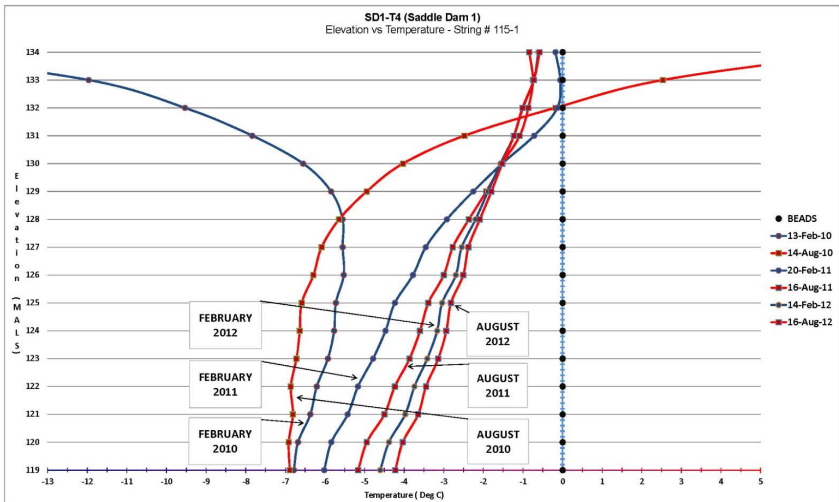
Figure 6: SD1-T4 Thermistor Results on Saddle Dam 1
