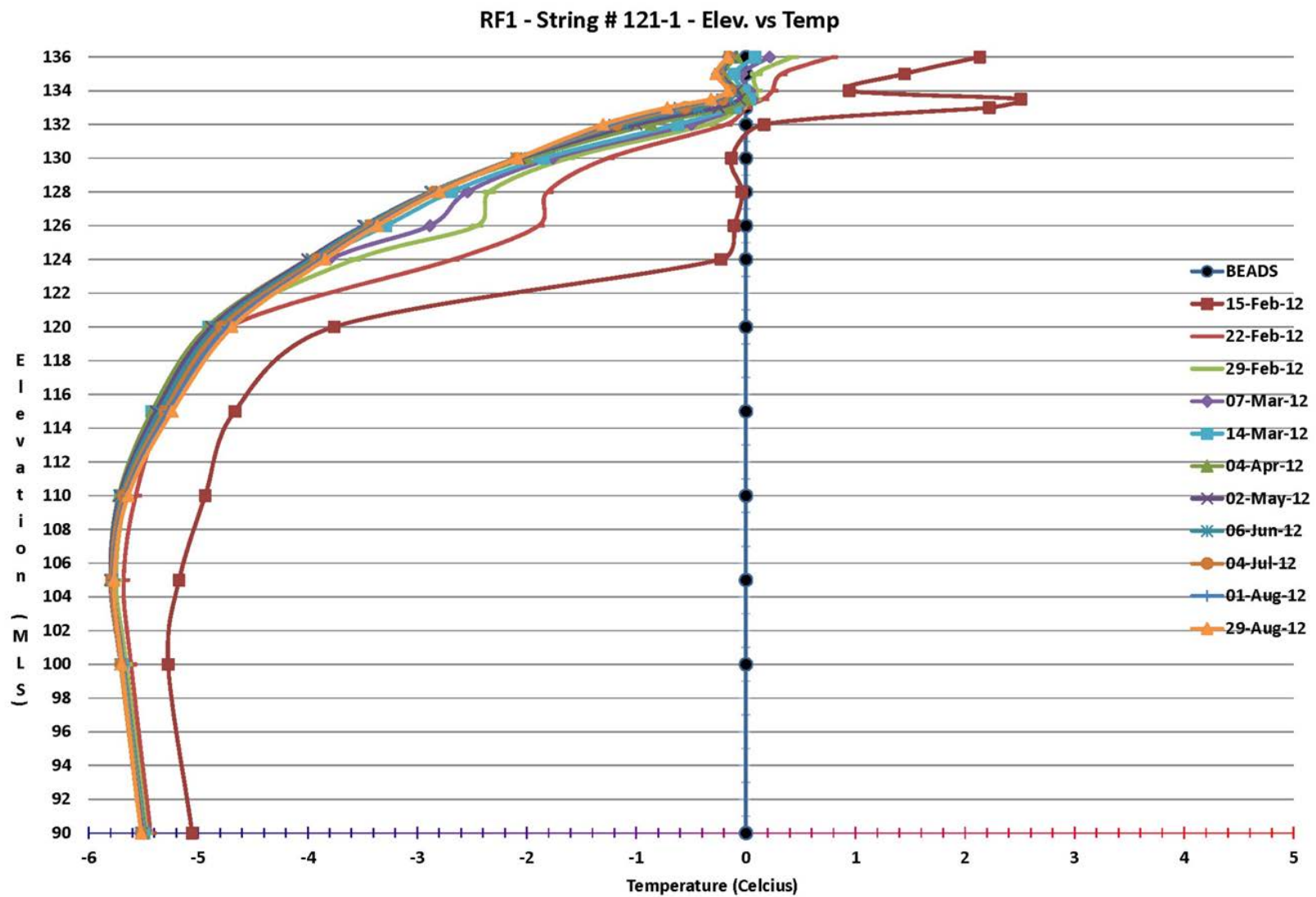
Figure 8: T121-1 Thermistor Results on RF1
