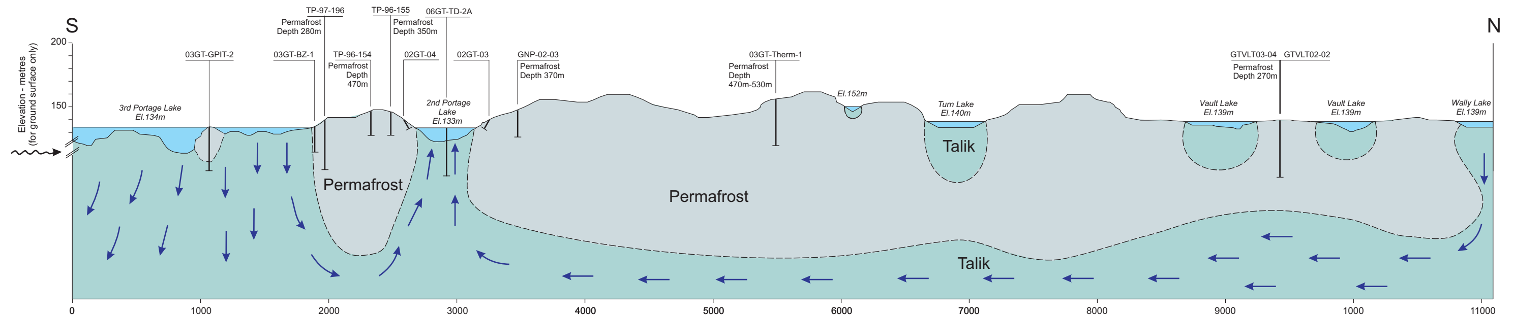
B CROSS SECTION B-B'
