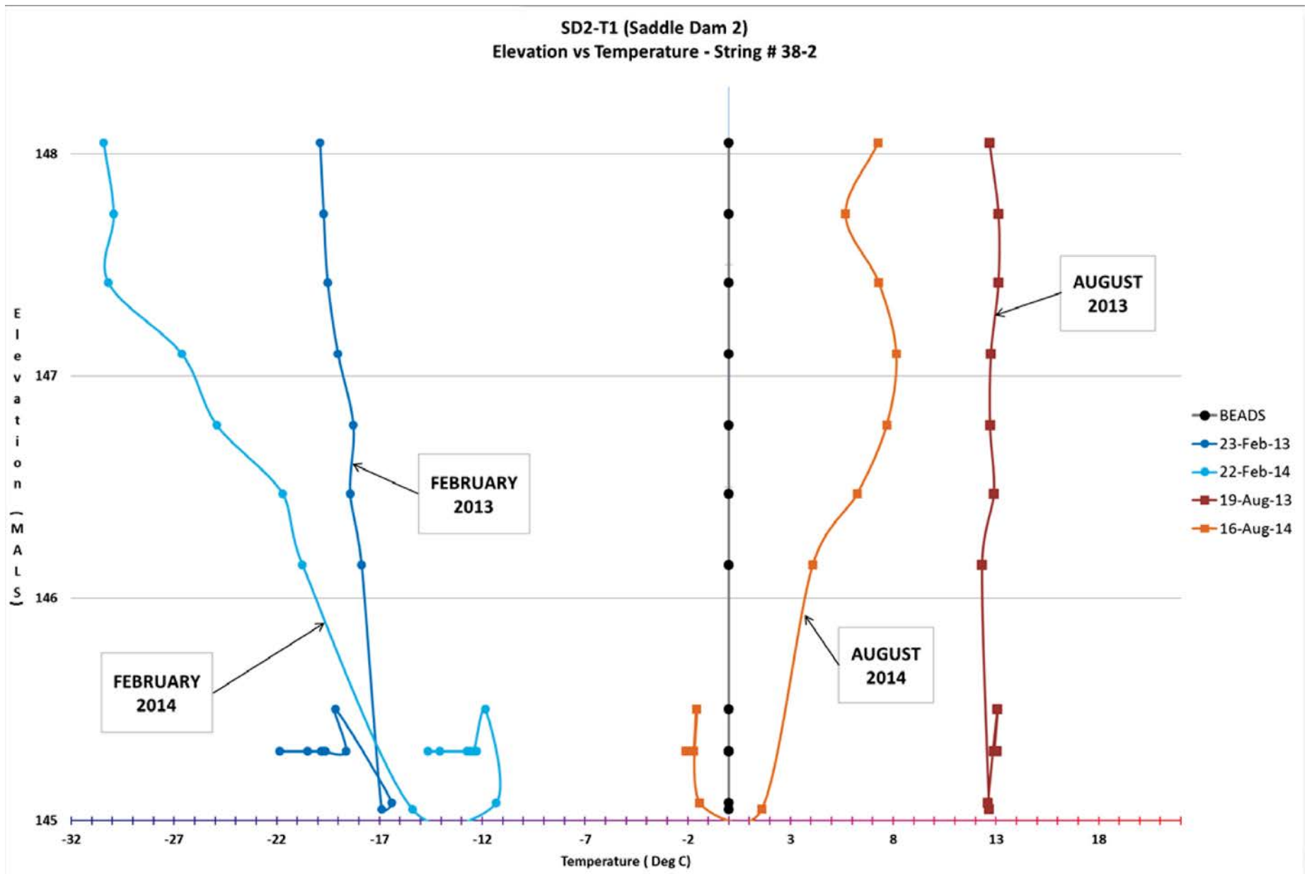
Figure 9 - Thermistor SD2-T1 on Saddle Dam 2
