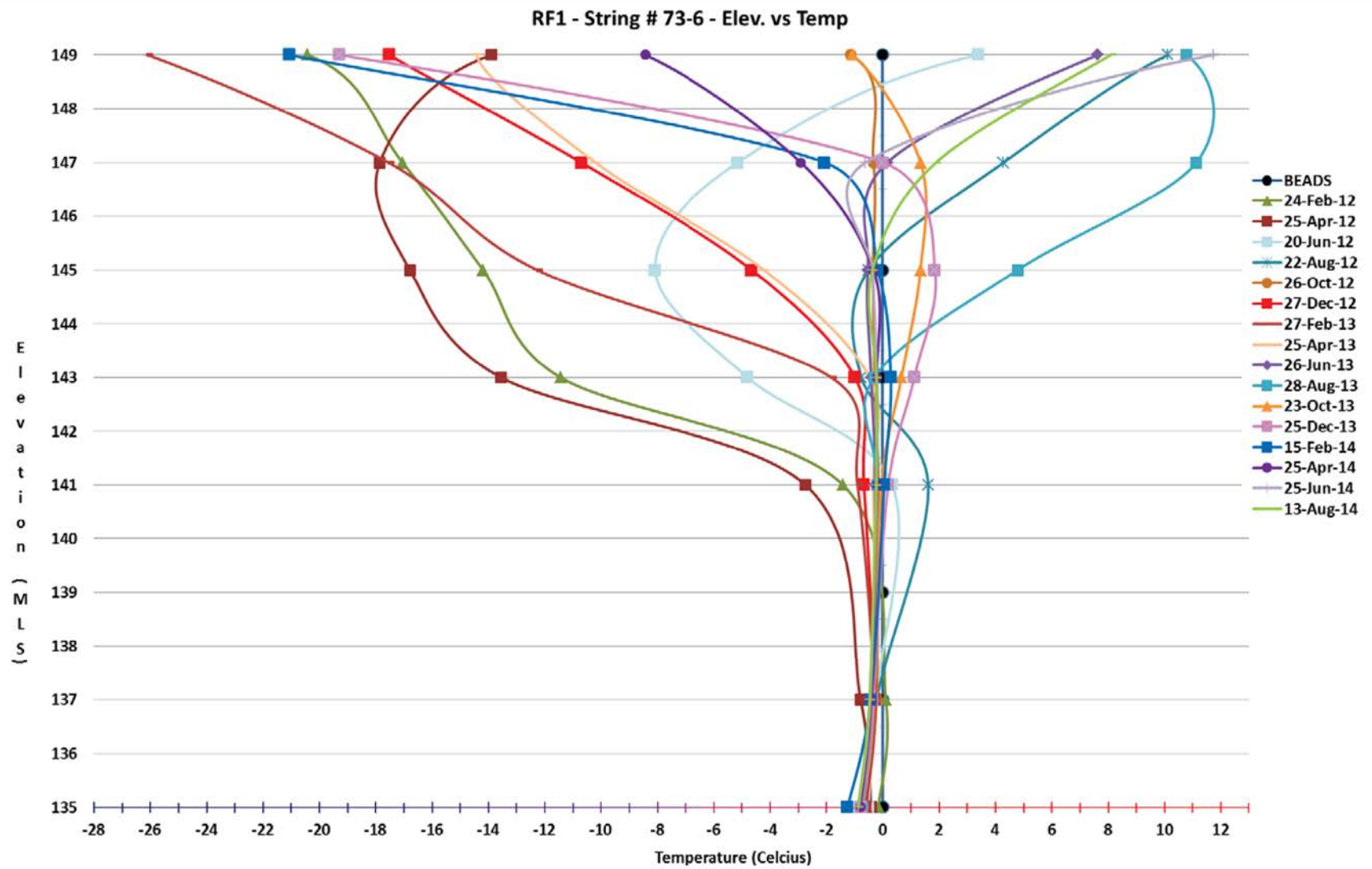
Figure 15 - Thermistor T73-6 on RF1
