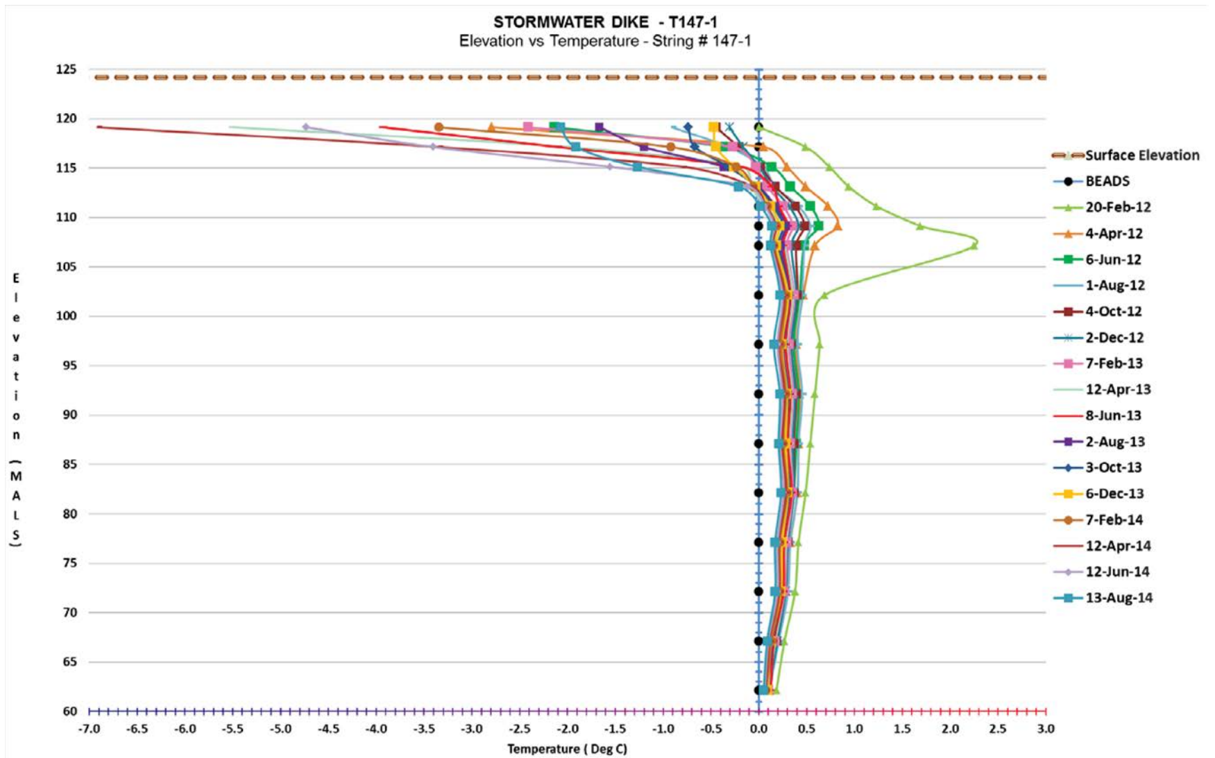
Figure 13 – Thermistor T147-1 on Stormwater Dike
