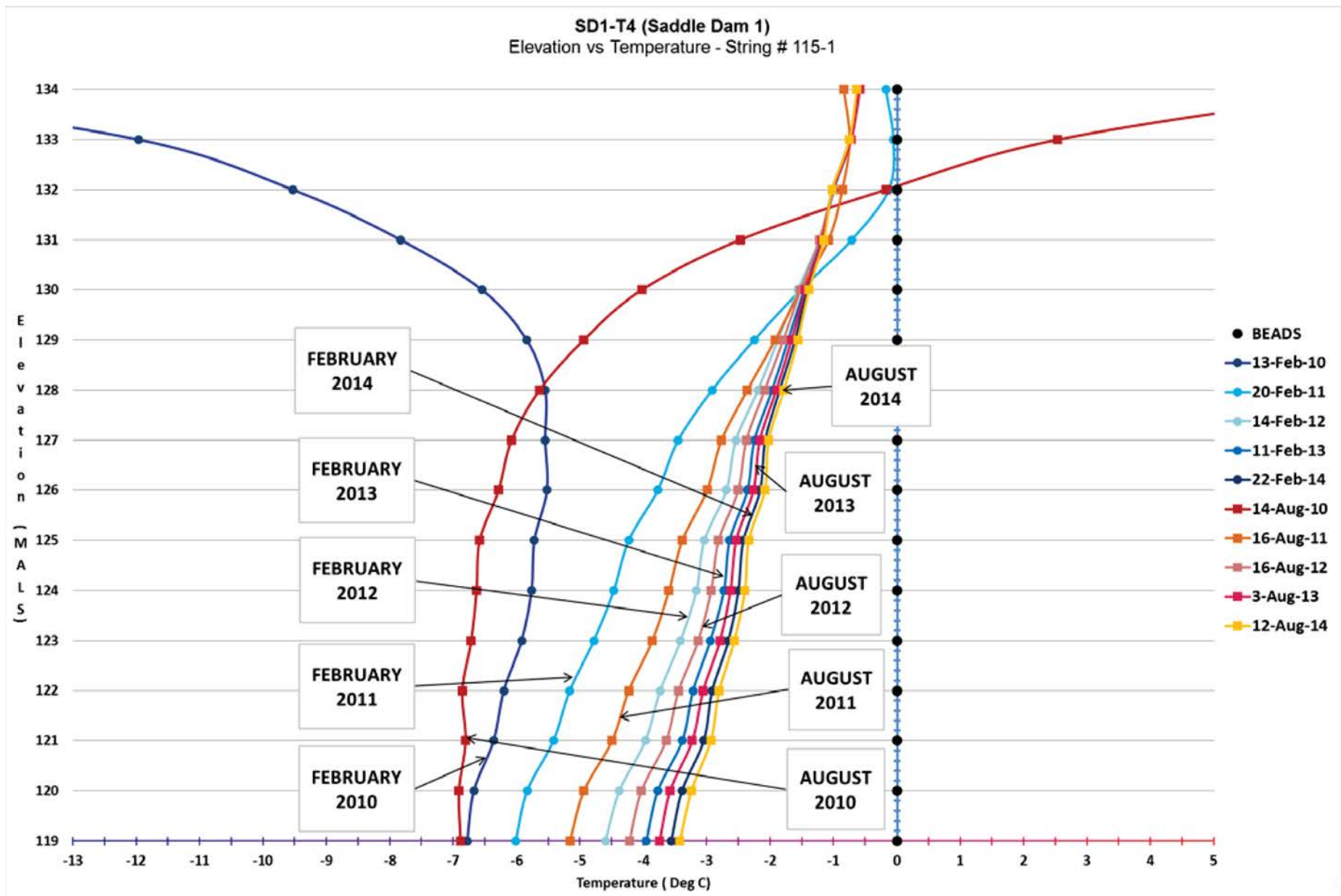
Figure 8 - Thermistor SD1-T4 on Saddle Dam 1
