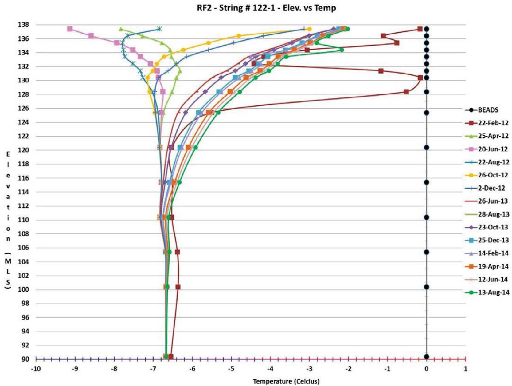
Figure 17 - Thermistor T122-1 on RF2
