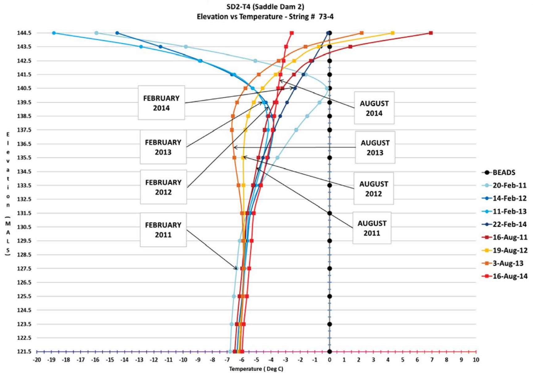
Figure 12 – Thermistor SD2-T4 on Saddle Dam 2
