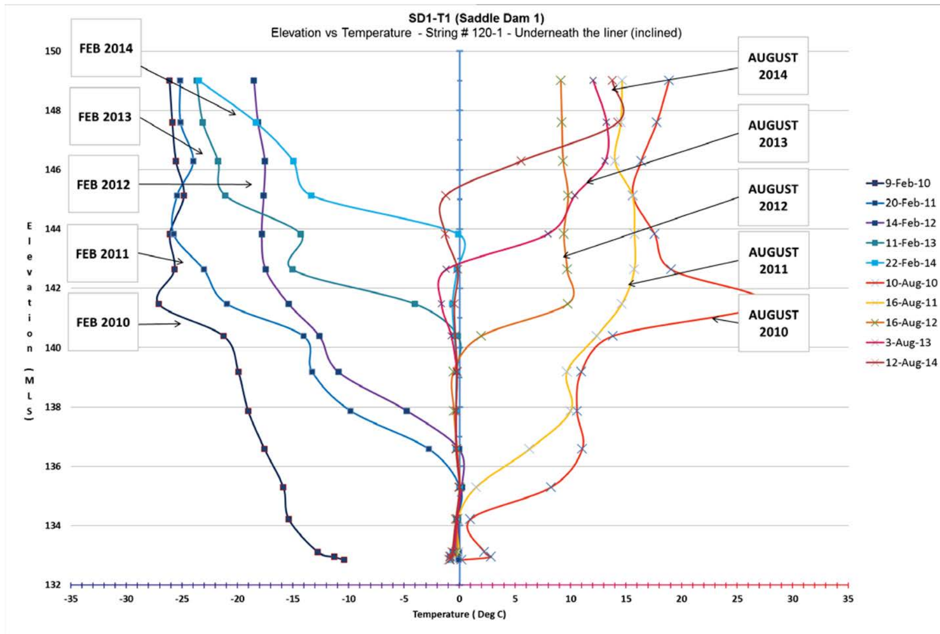
Figure 5 – Thermistor SD1-T1 on Saddle Dam 1
