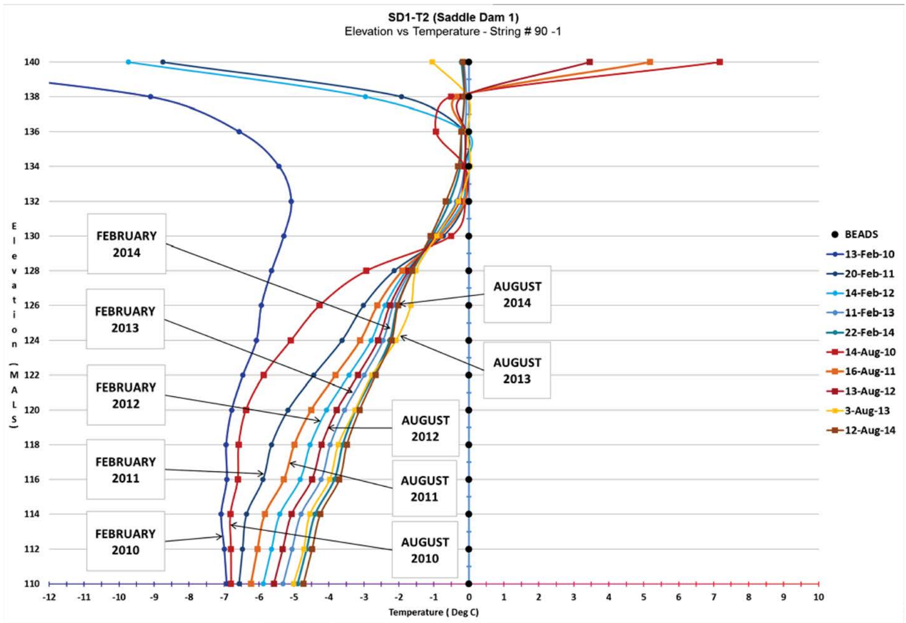
Figure 6 - Thermistor SD1-T2 on Saddle Dam 1
