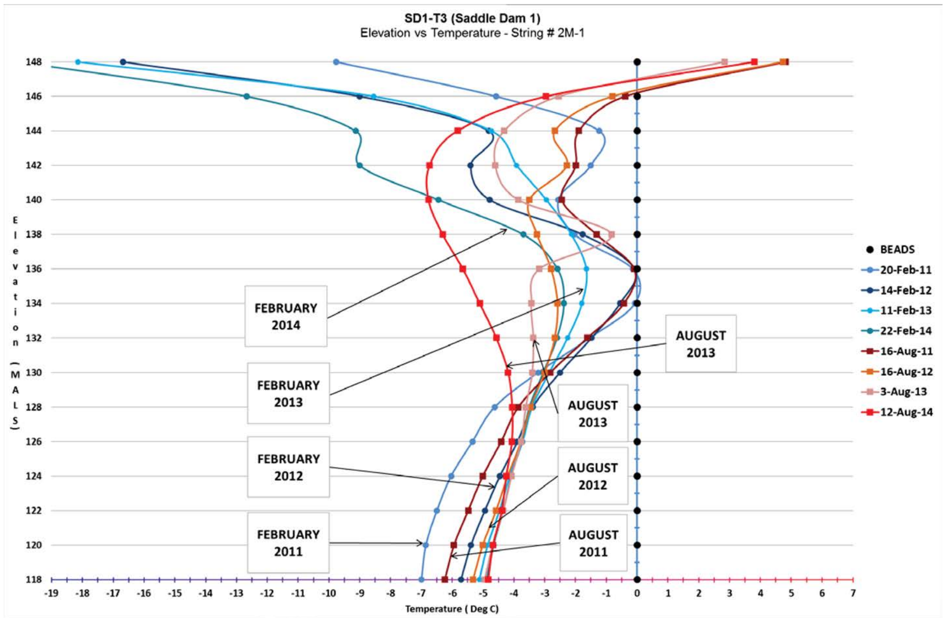
Figure 7 – Thermistor SD1-T3 on Saddle Dam 1
