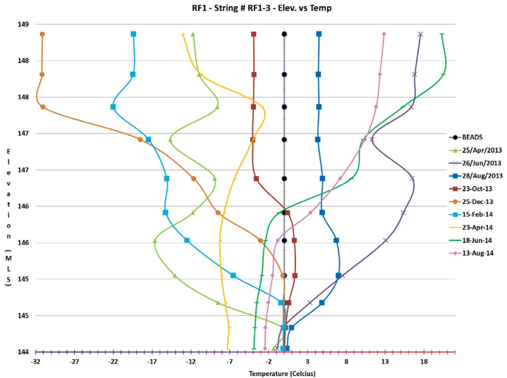
Figure 16 - Thermistor RF1-3 on RF1
