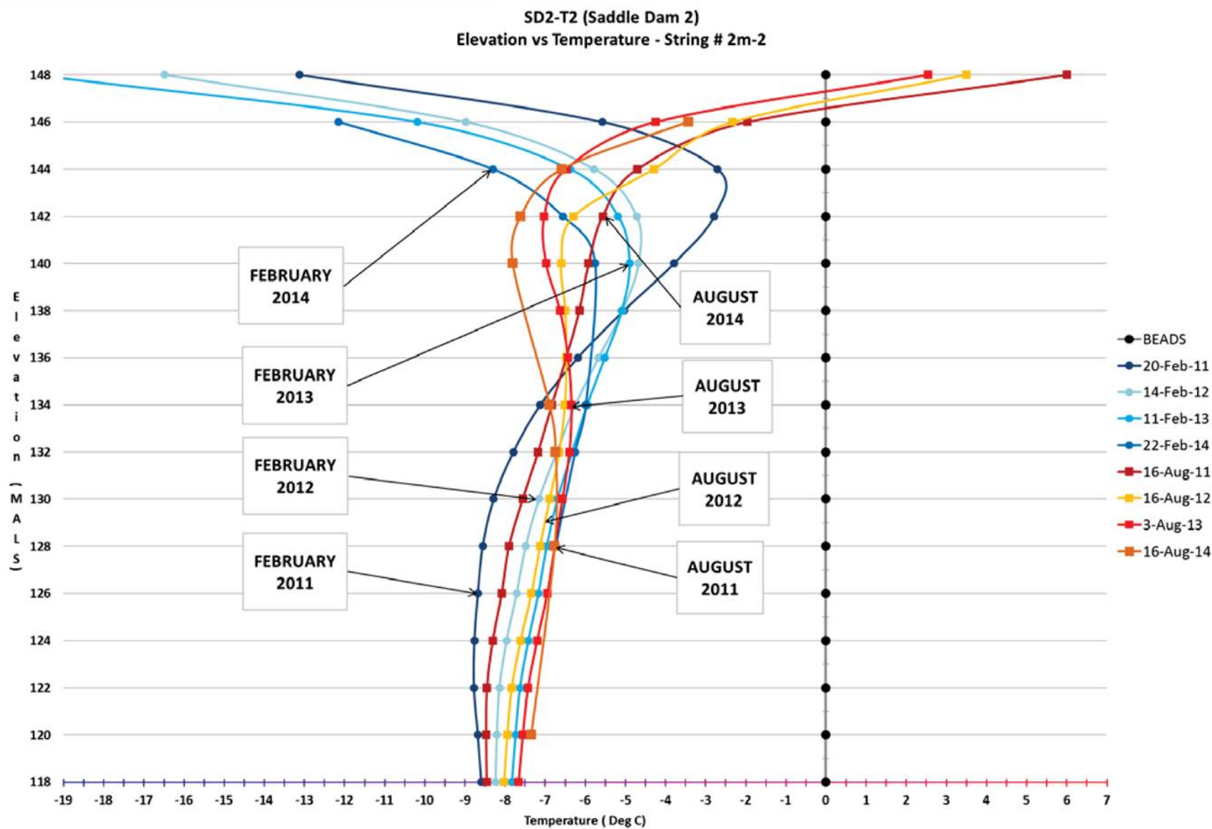
Figure 10 – Thermistor SD2-T2 on Saddle Dam 2
