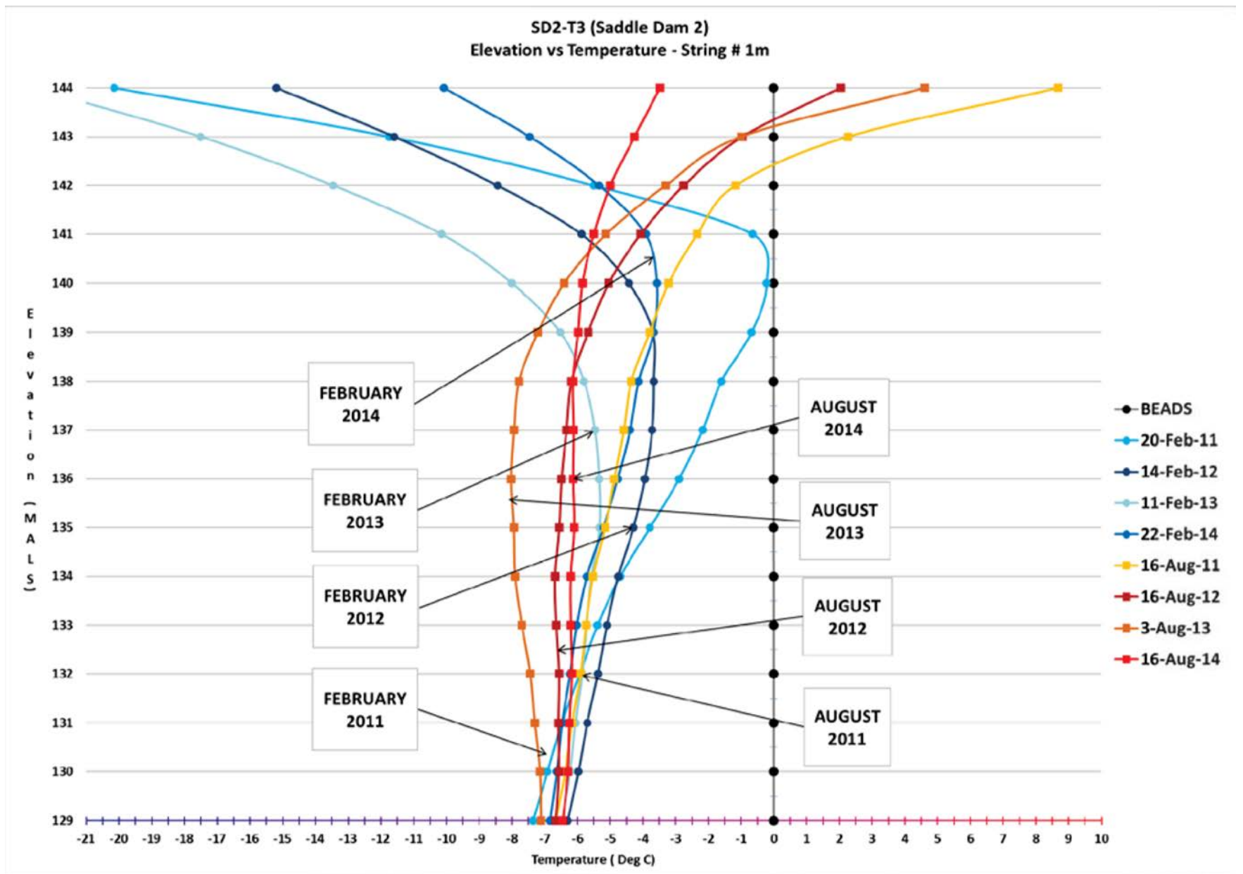
Figure 11 – Thermistor SD2-T3 on Saddle Dam 2
