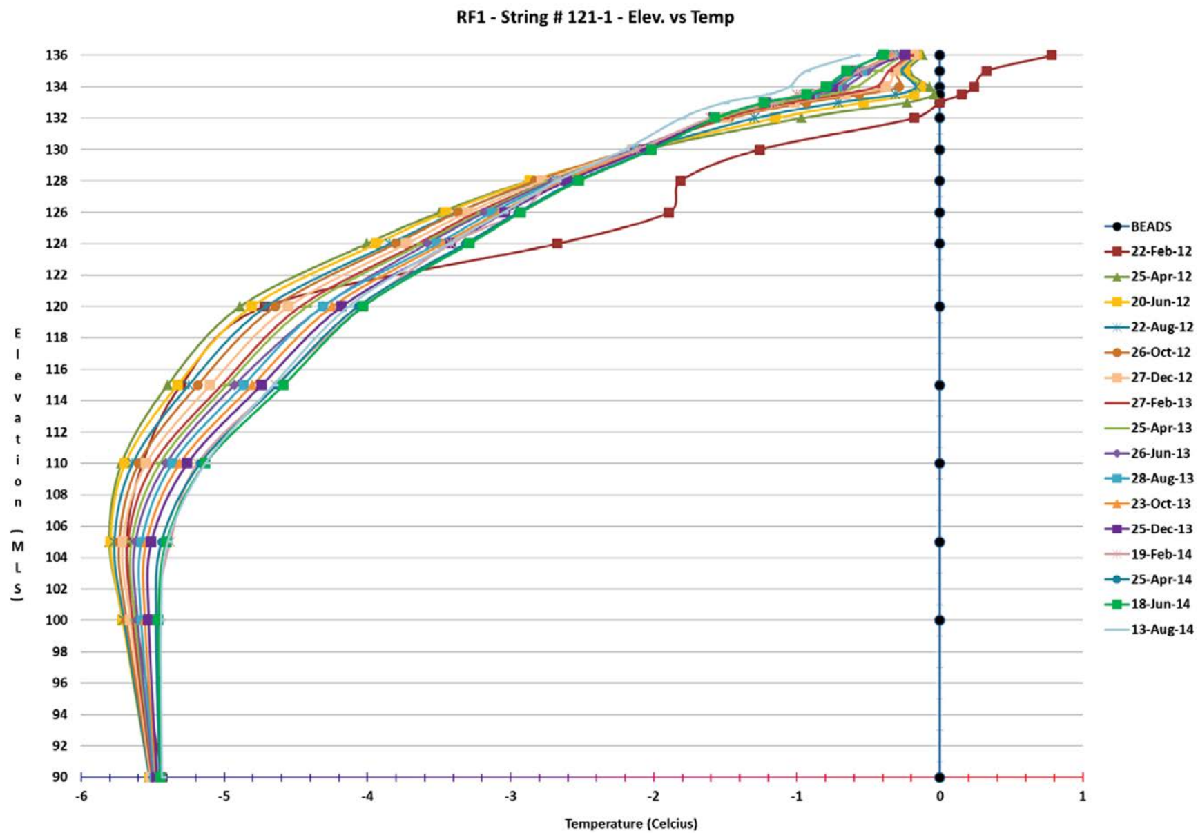
Figure 14 - Thermistor T121 on RF1
