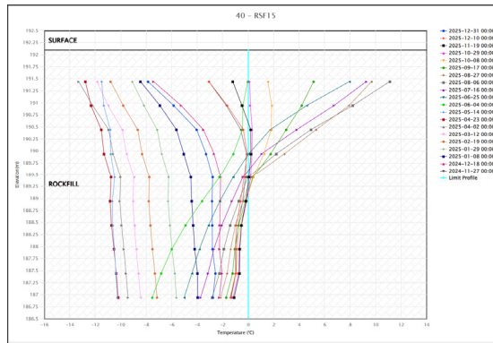
Temperature(°C): RSF-15
