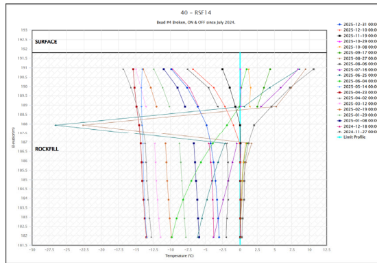
Temperature(°C): RSF-14
