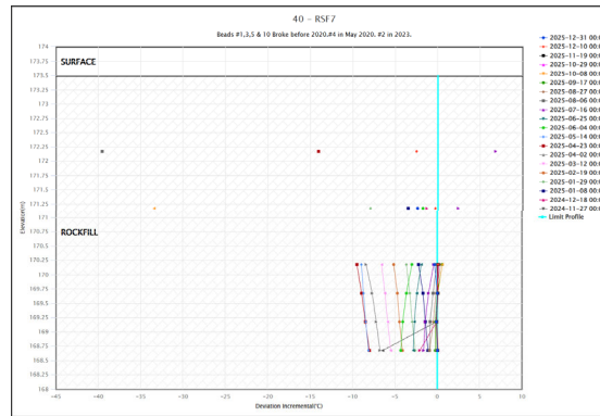
Temperature(°C): RSF-07
