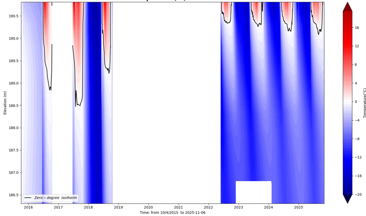
Temperature(°C): RSF-13
