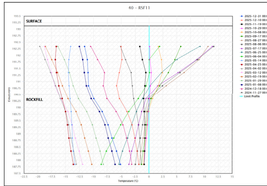
Temperature(°C): RSF-11
