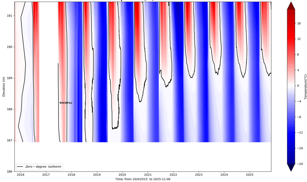
Temperature(°C): RSF-15
