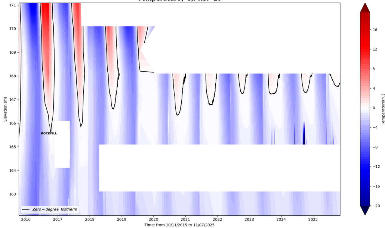
Temperature(°C): RSF-10
