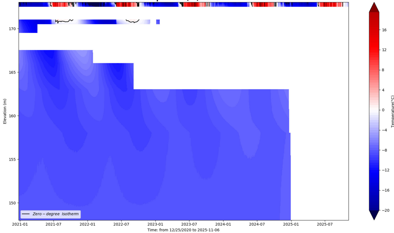
Temperature(°C): RSF18
