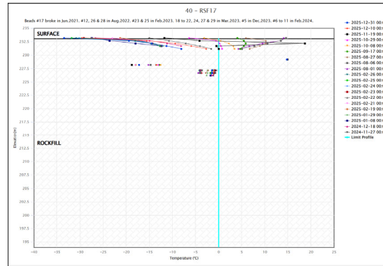
Temperature(°C): RSF17
