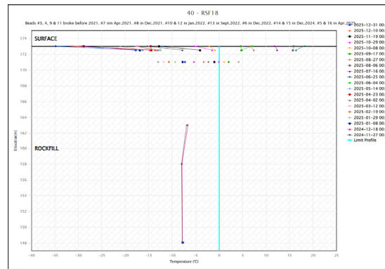
Temperature(°C): RSF18
