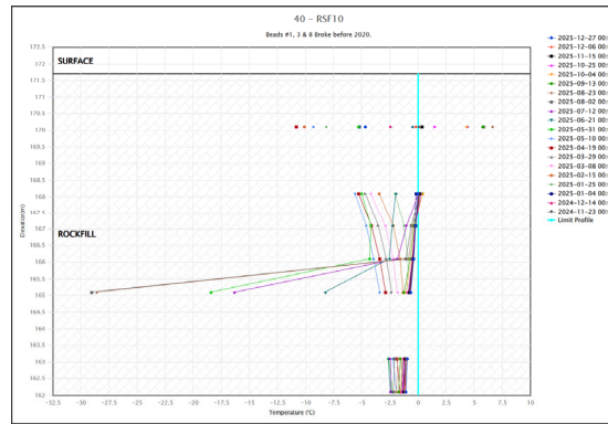
Temperature(°C): RSF-10
