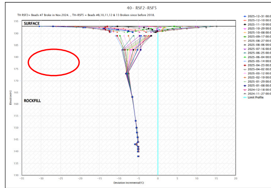
Temperature(?C): RSF-05
