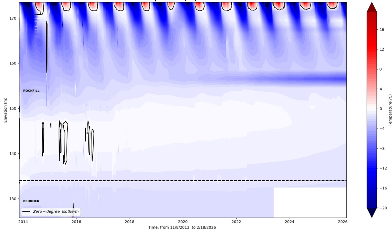
Temperature(°C): RSF-03
