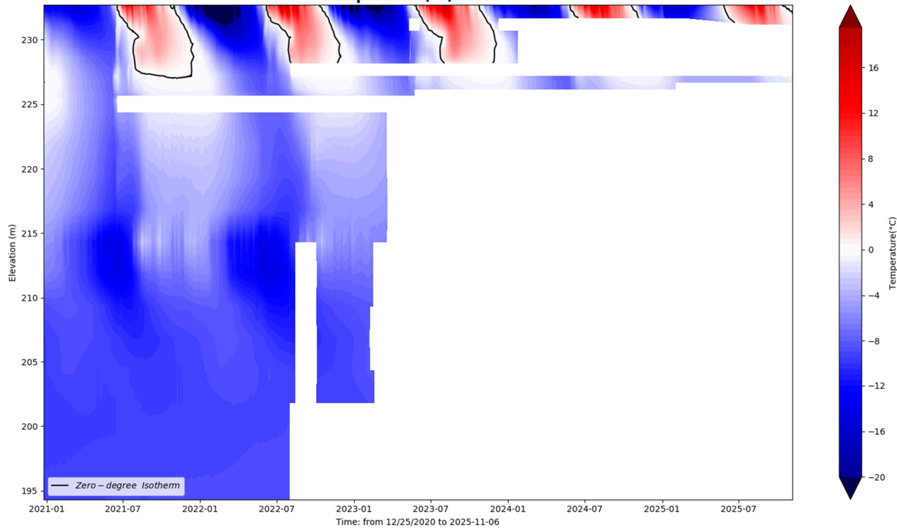
Temperature(°C): RSF17
