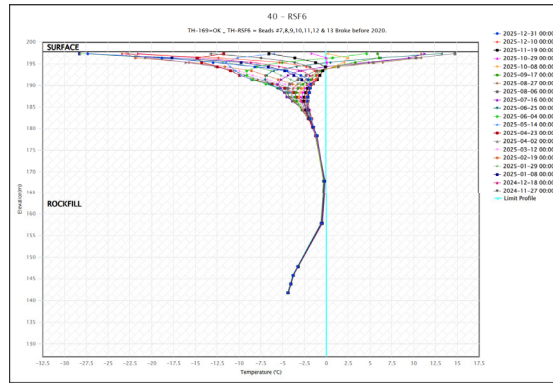
Temperature(°C): RSF-06
