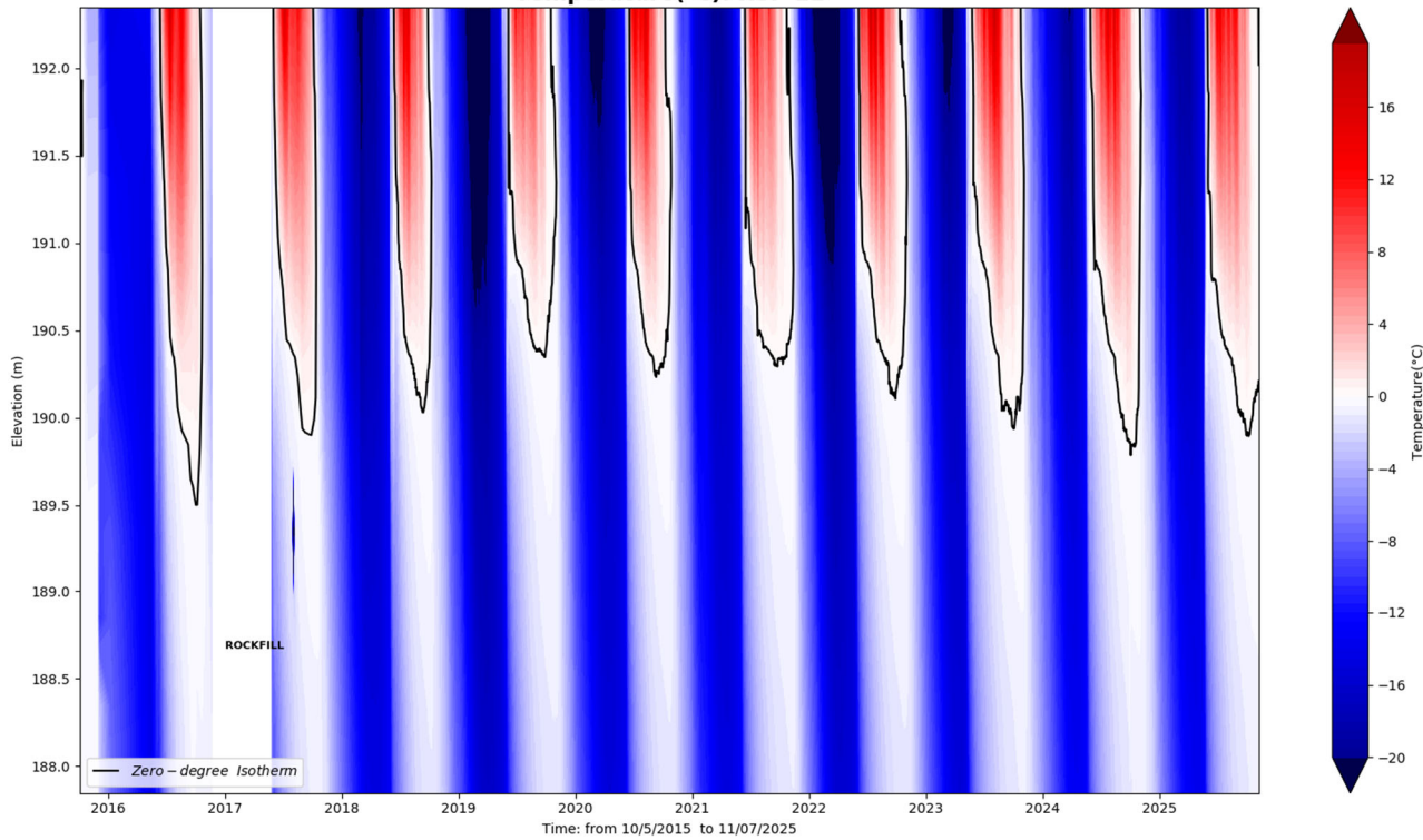
Temperature(°C): RSF-11
