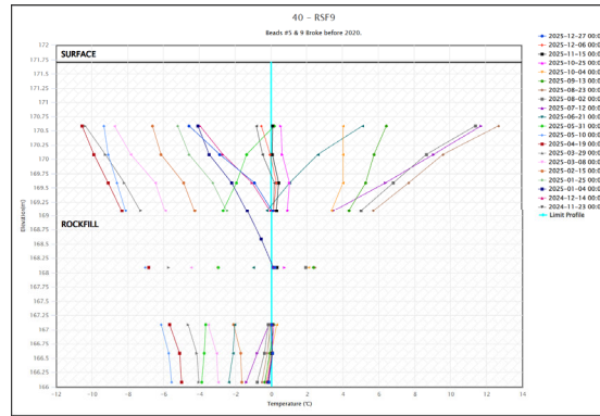
Temperature(°C): RSF-09
