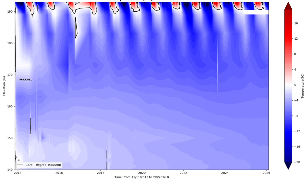
Temperature(?C): RSF-05
