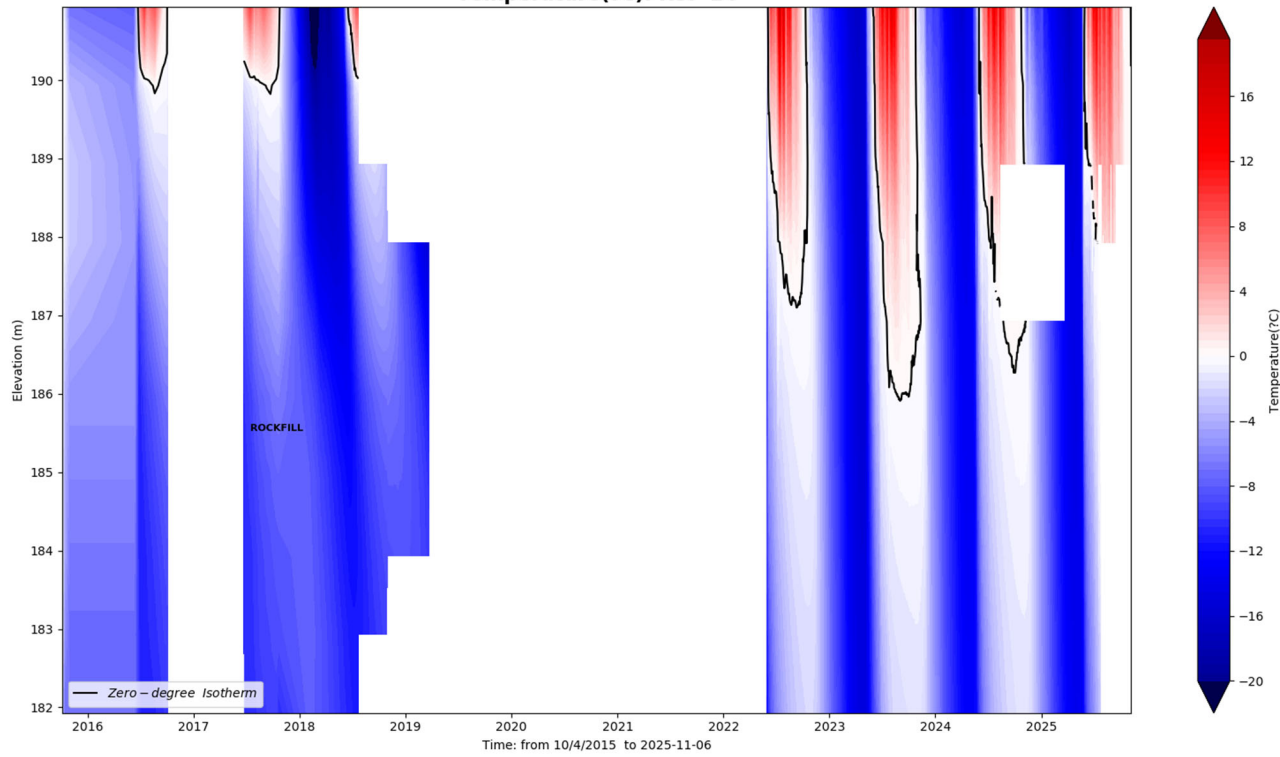
Temperature(°C): RSF-14
