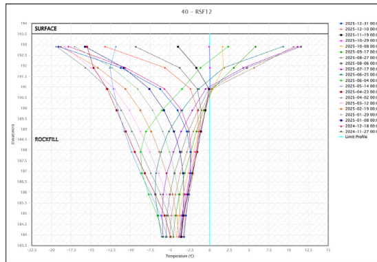
Temperature(°C): RSF-12
