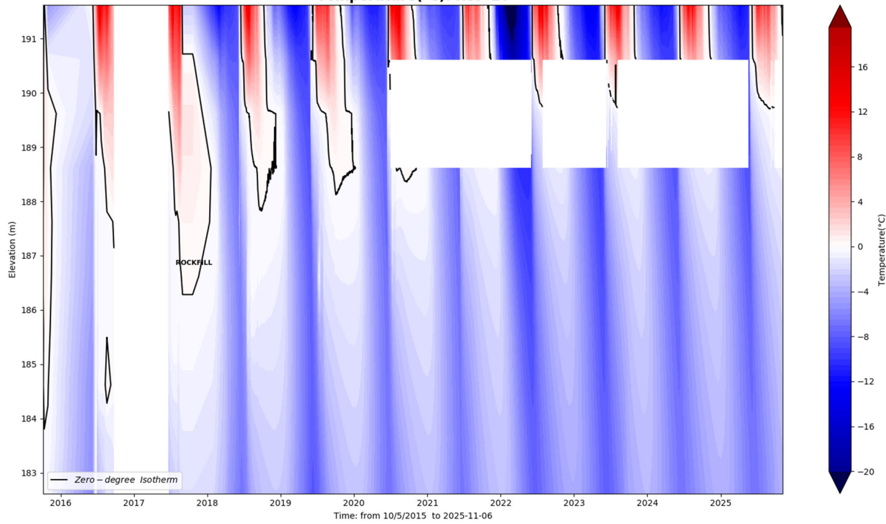
Temperature(°C): RSF-16
