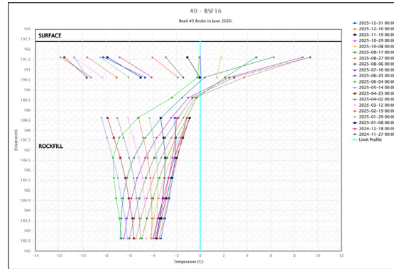
Temperature(°C): RSF-16
