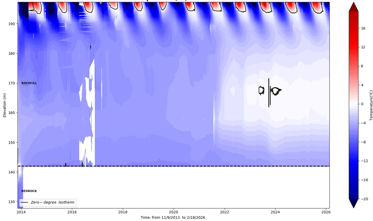
Temperature(°C): RSF-06
