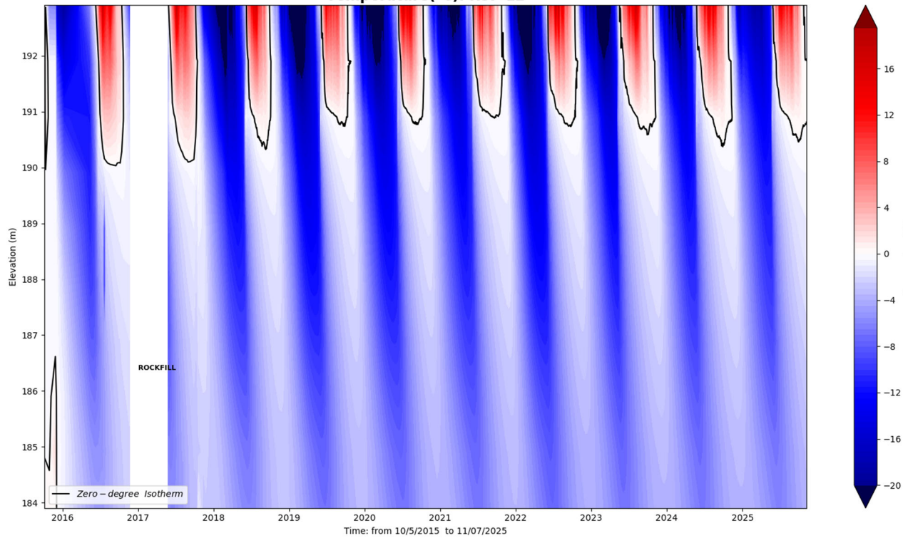
Temperature(°C): RSF-12
