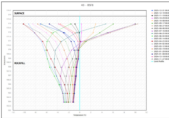
Temperature(°C): RSF-08
