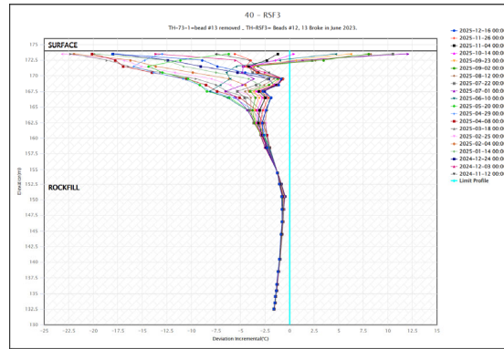
Temperature(°C): RSF-03
