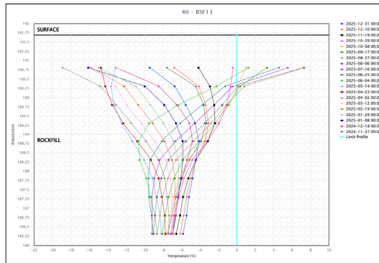
Temperature(°C): RSF-13
