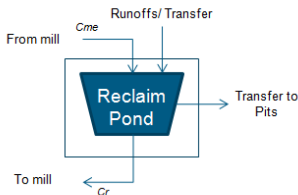
Figure 3-1: Mass balance for dissolved metals, nitrate and cyanide
