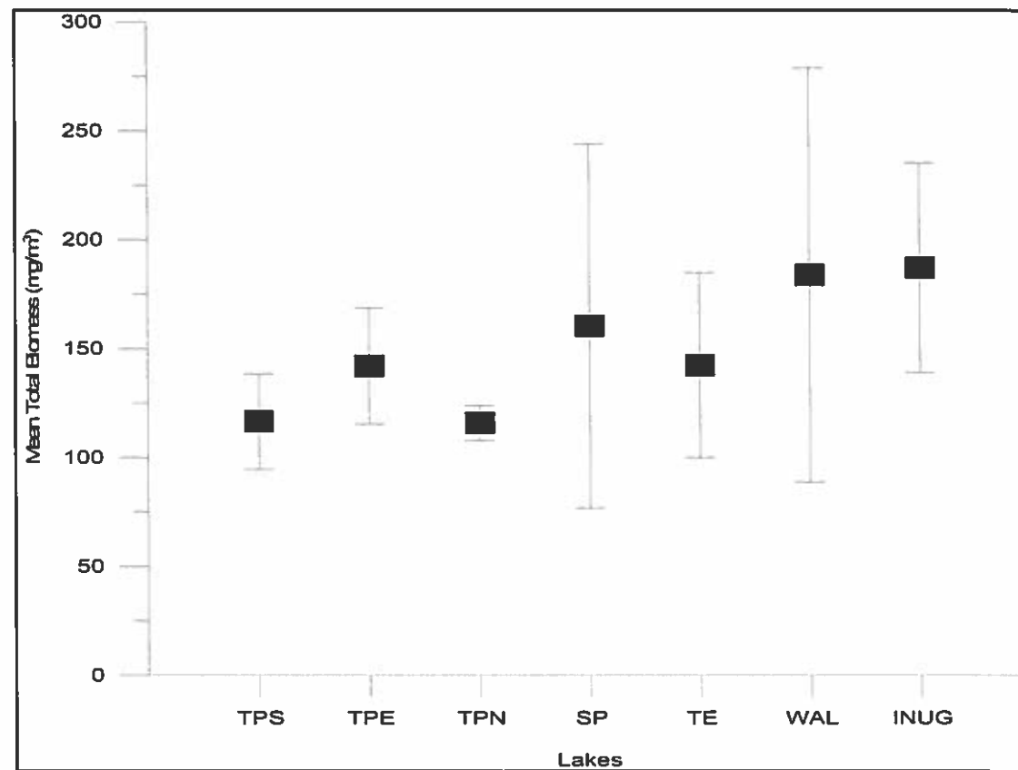
Figure 3-9: Phytoplankton Mean Total Biomass, +/- 1 Standard Deviation, Meadowbank Study Lakes, 2006.
