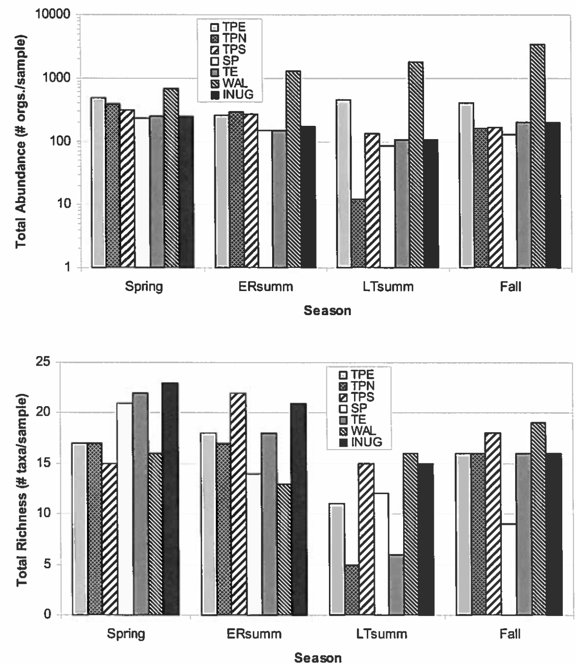
Figure 3-12: Benthic Invertebrate Total Abundance (top) and Total Richness (bottom) for each season, 2006.
