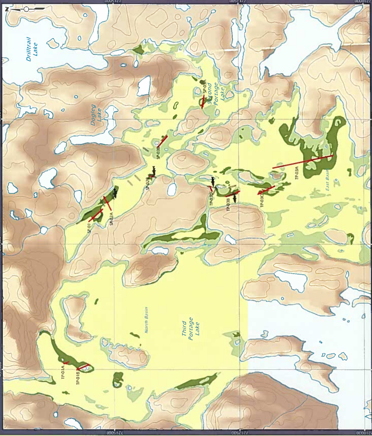
Figure 3-16: Transect and Gillnet Locations, Fish Spawning Survey, 2006, with Relative Value of Fish Habitat
