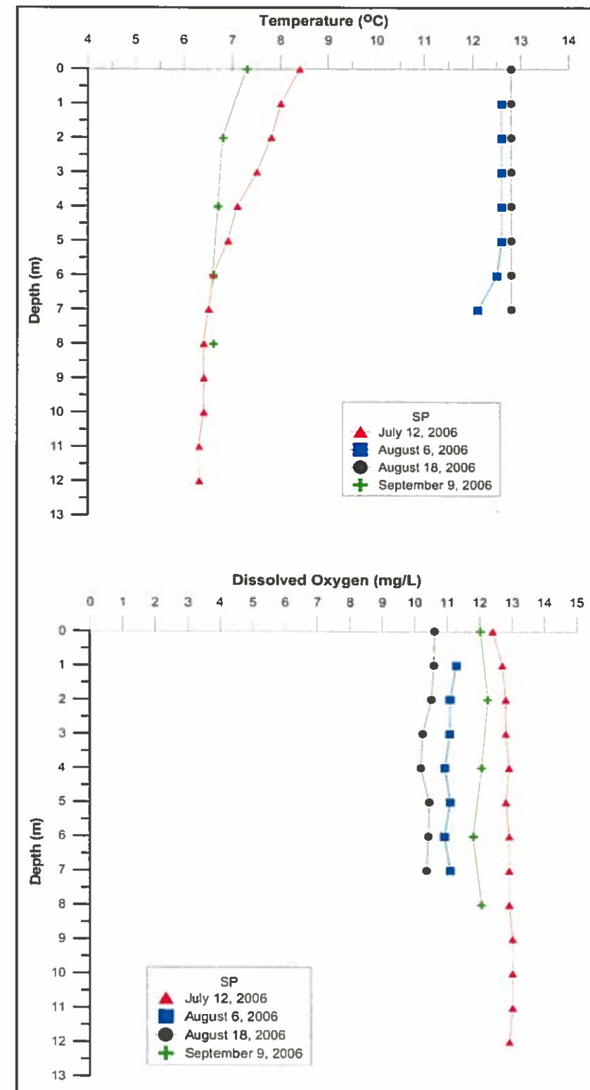
Figure 3-5: Temperature ( ^{\circ}\text{C} ) and Dissolved Oxygen (mg/L) Profiles for Second Portage Lake, 2006.
