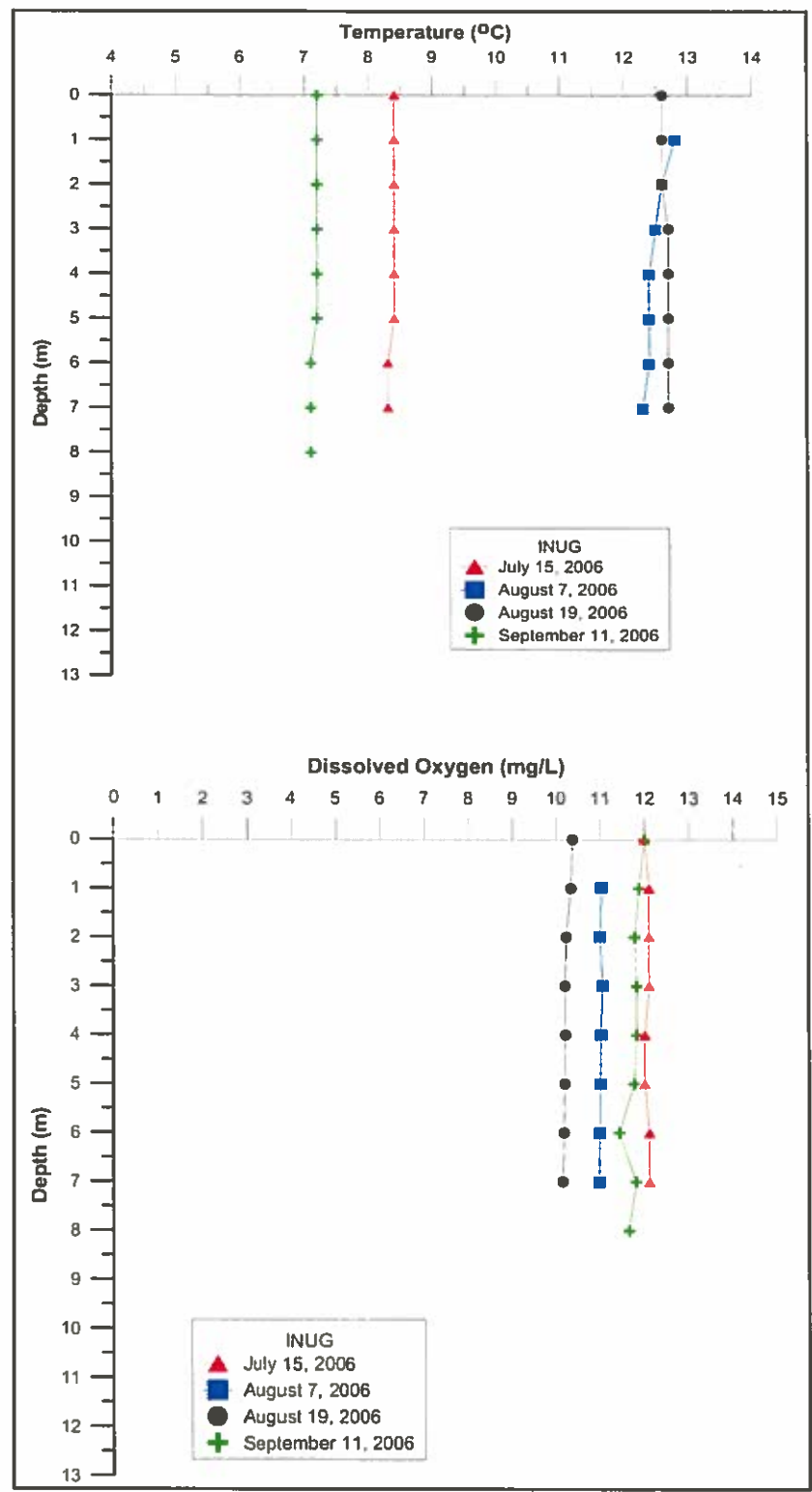
Figure 3-7: Temperature ( ^{\circ}\text{C} ) and Dissolved Oxygen ( \text{mg/L} ) Profiles for Inuggugayualik Lake, 2006.
