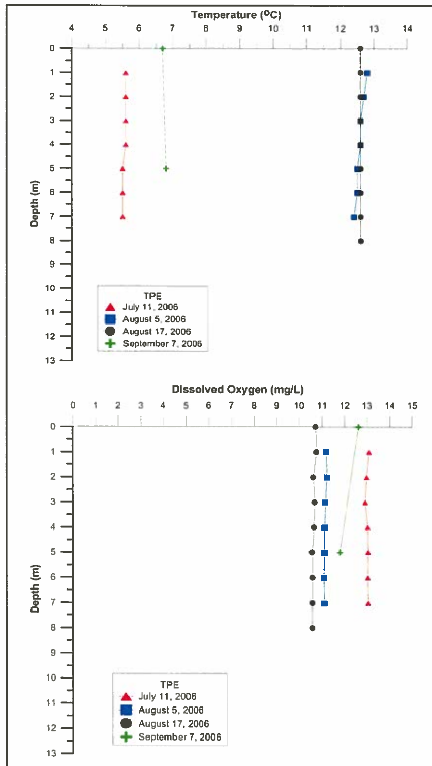
Figure 3-1: Temperature ( ^{\circ}\text{C} ) and Dissolved Oxygen (mg/L) Profiles for Third Portage Lake – East Basin, 2006.
