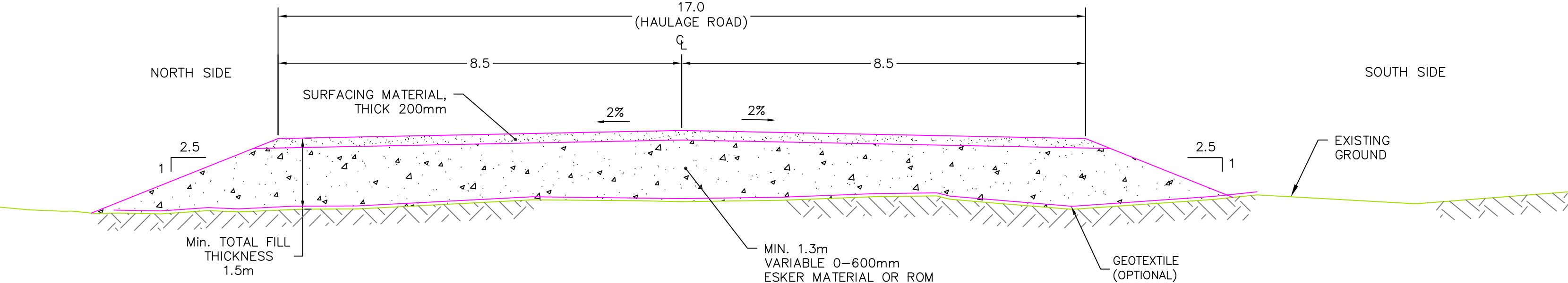
TYPICAL CROSS SECTION ~ AWAR - WITH EMBANKMENT - <= 3.0m (FZONE, PUMP ZONE, WESTMEG AND NORMEG)
