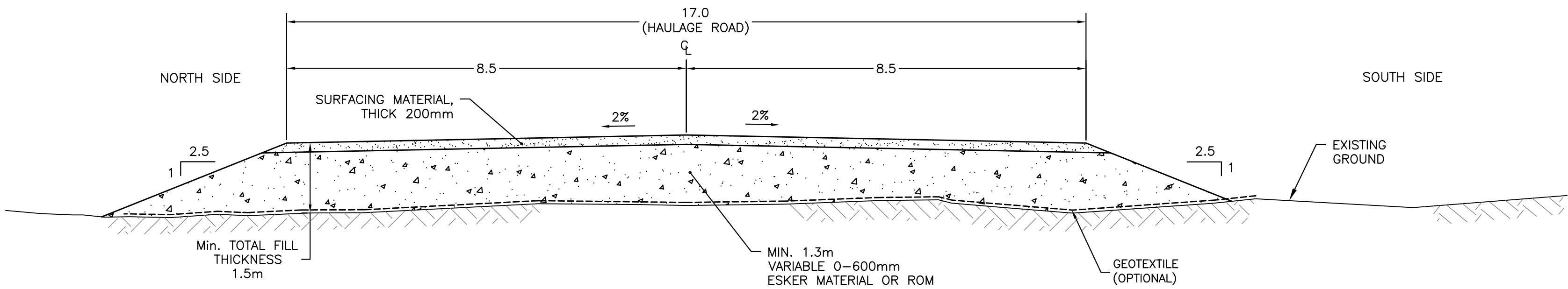
TYPICAL CROSS SECTION ~ AWAR - WITH EMBANKMENT - <= 3.0m (DISCOVERY ROAD JUNCTION TO DICOVERY SITE, FZONE, PUMP ZONE, WESTMEG AND NORMEG) Éch: 1: 75
