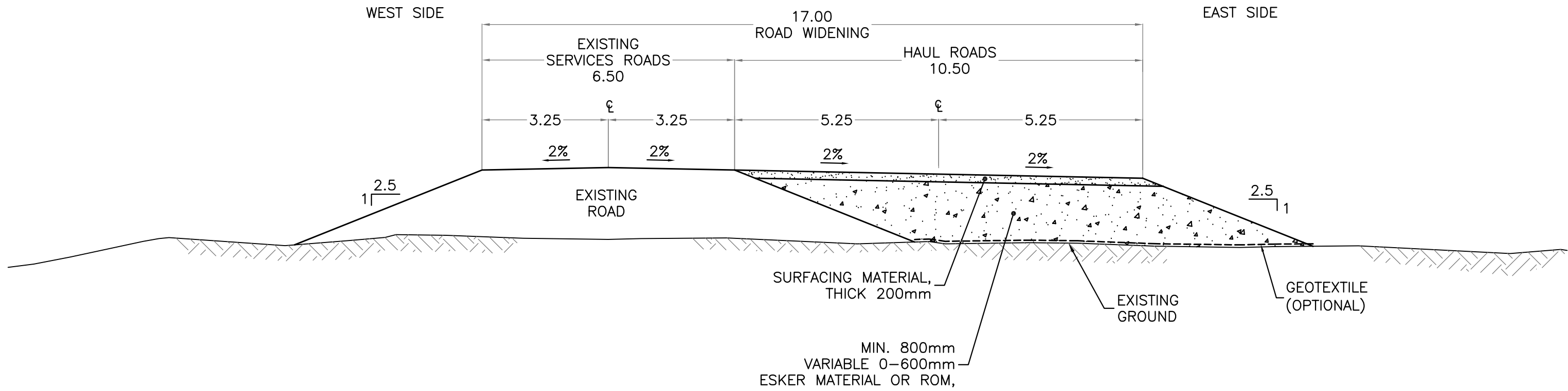
TYPICAL CROSS SECTION ~ AWAR - WITH EMBANKMENT < 3.0m (DISCOVERY ROAD JUNCTION TO MELIADINE MAIN SITE) Éch: 1:100
