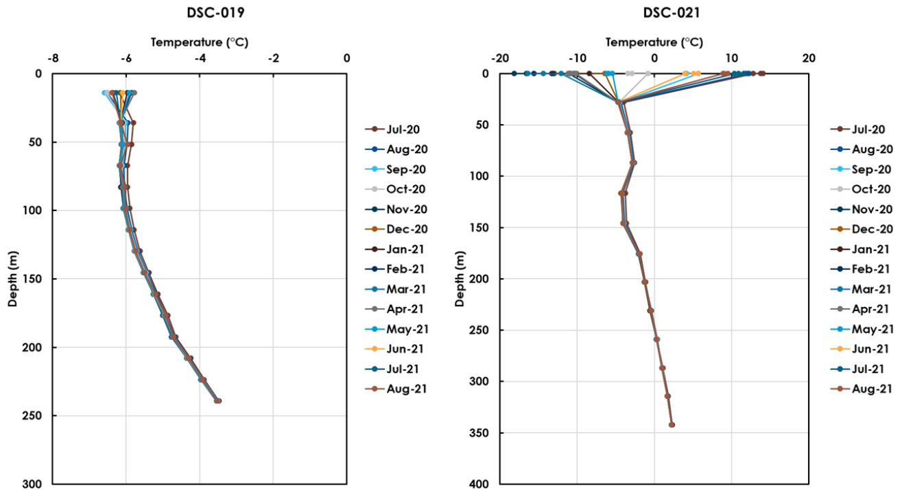
Figure 3.7: Bedrock temperatures measured within the footprint of the Discovery WRSF.
