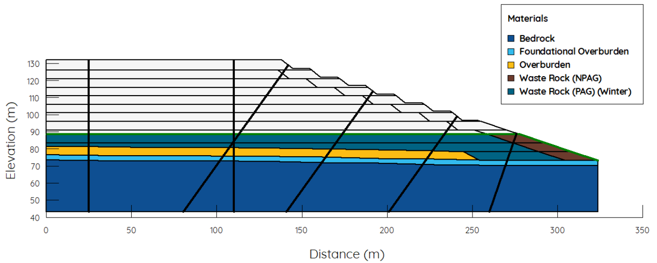
Figure B.3: Meliadine Discovery WRSF construction – Winter Year 1.
