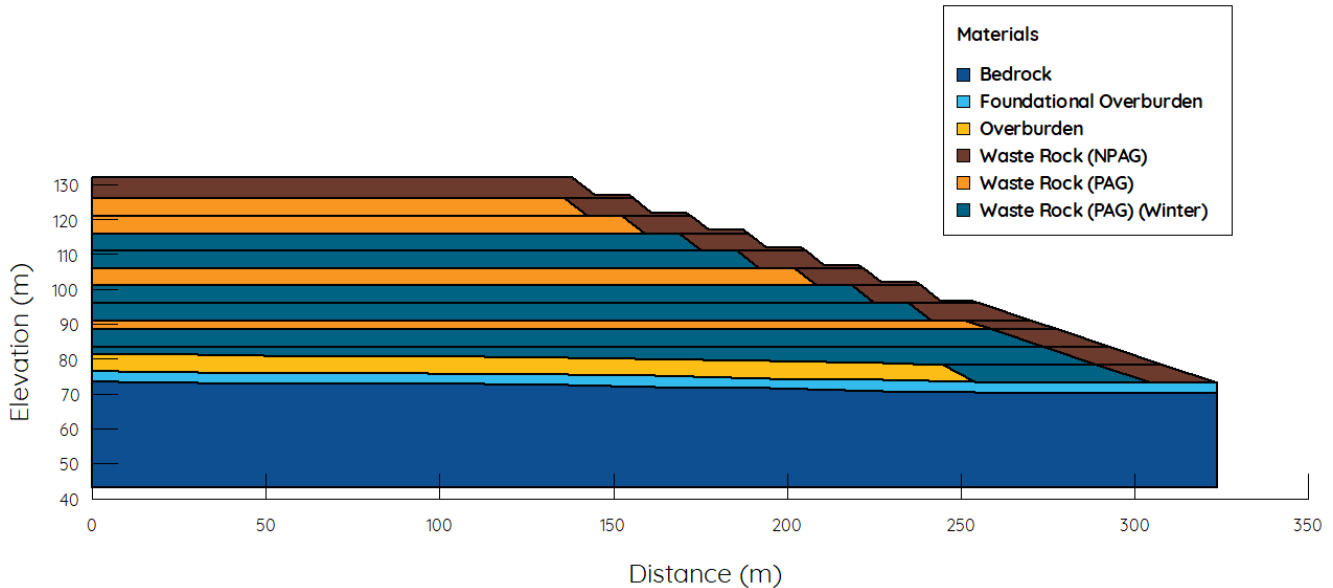
Figure 3.6: Idealized southwest facing cross-section of Meliadine Discovery WRSF (adapted from Tetra Tech, 2022).
