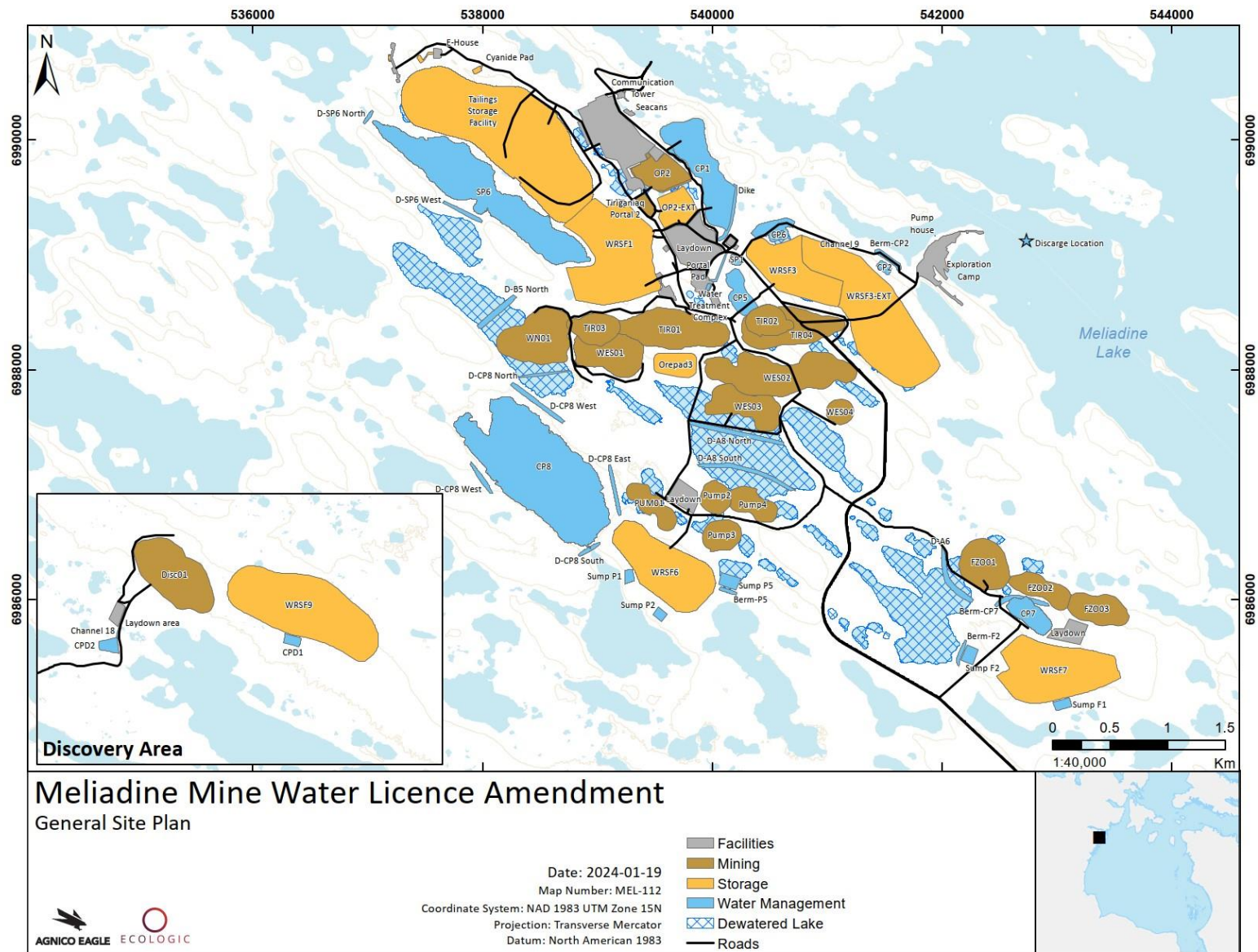
Figure 2.1 : Meliadine Mine site layout.
