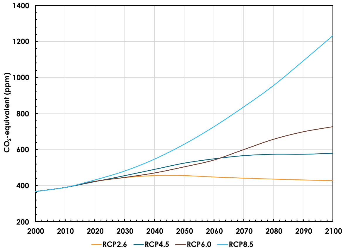
Figure 3.1: All forcing agents' atmospheric CO 2 -equivalent concentrations according to the four RCP scenarios.
