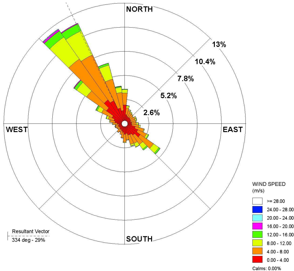
Figure 3.5: Wind rose for Meliadine site climate station.
