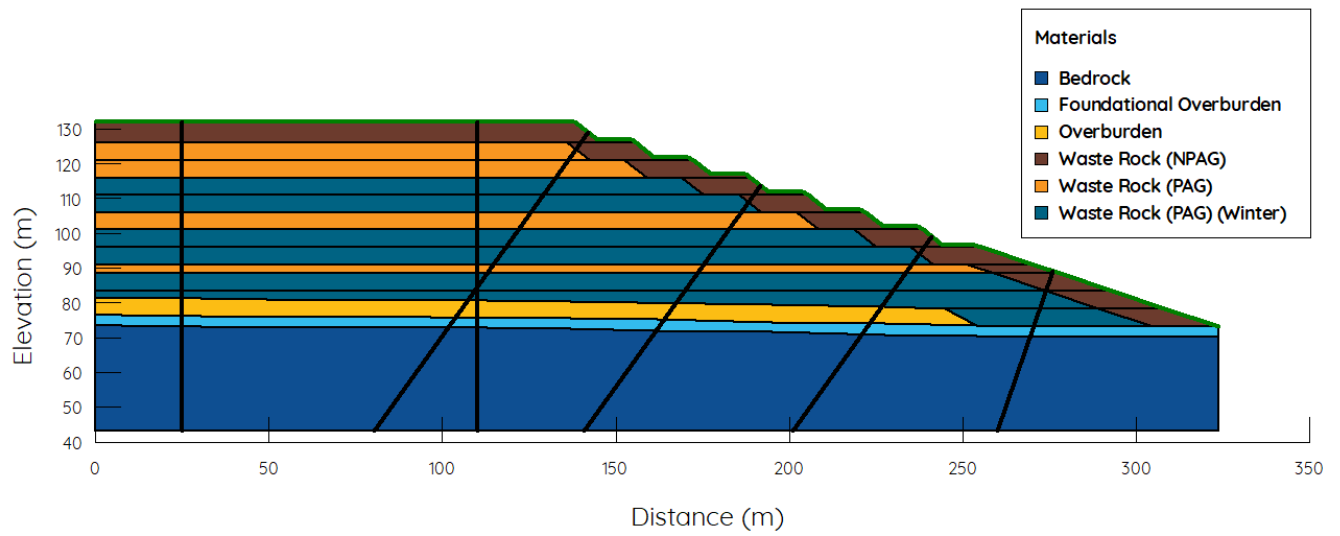
Figure B.8: Meliadine Discovery WRSF construction – Summer Year 3.
