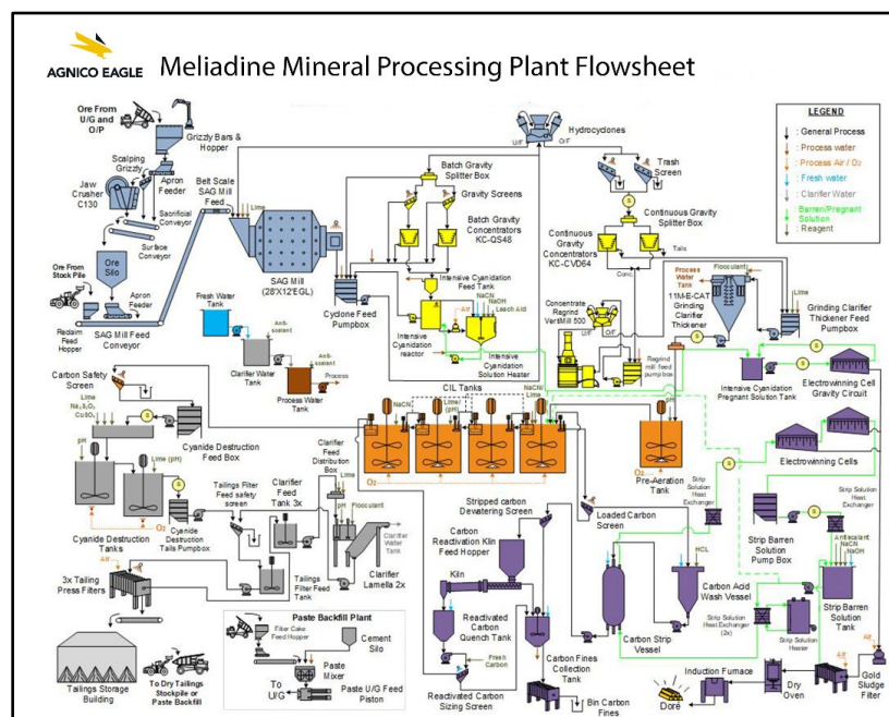
Figure 4-5 : Meliadine Mineral Processing Flowsheet
