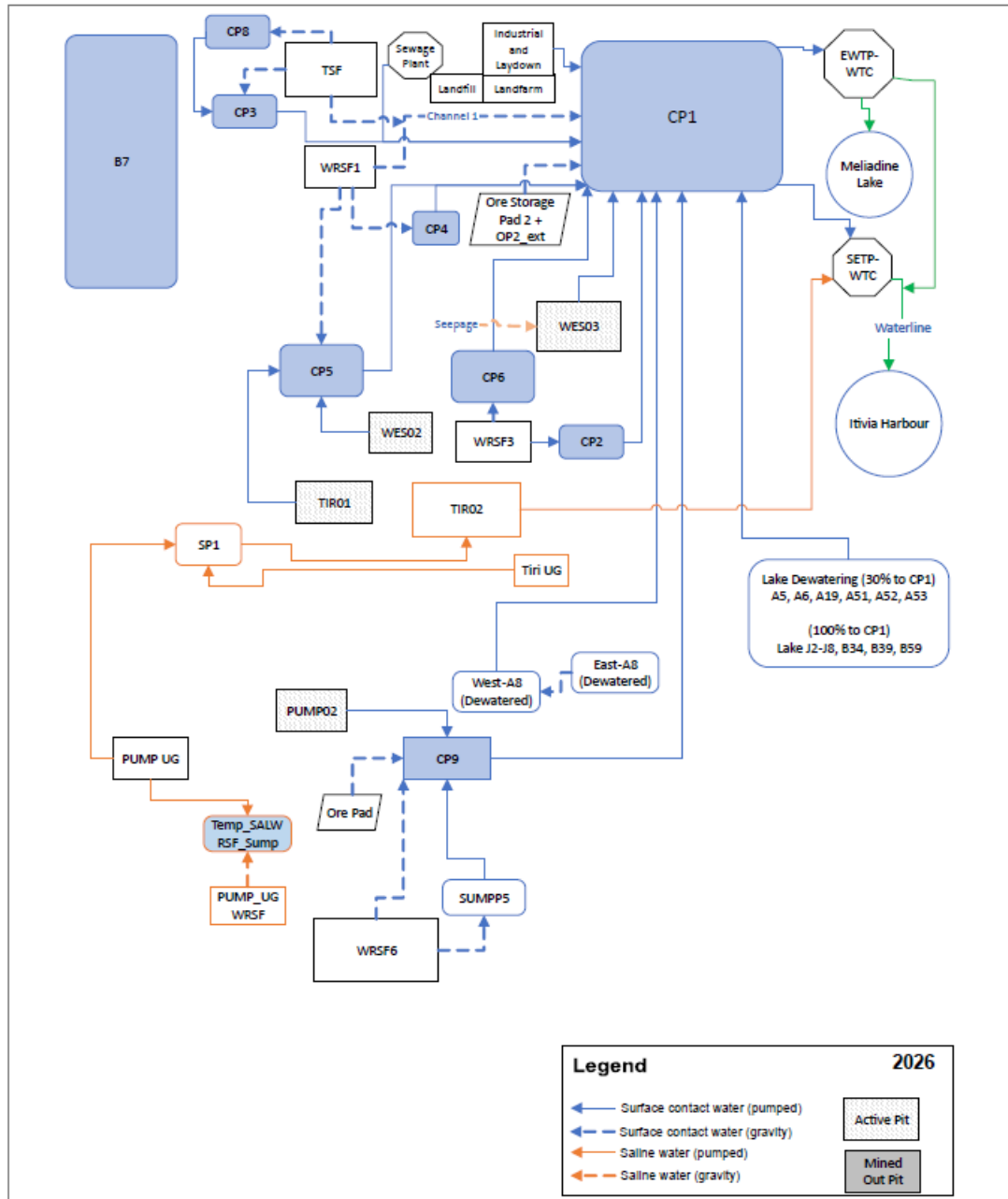
Figure 6: Conceptual Site Water Management Flow Diagram for the Site
