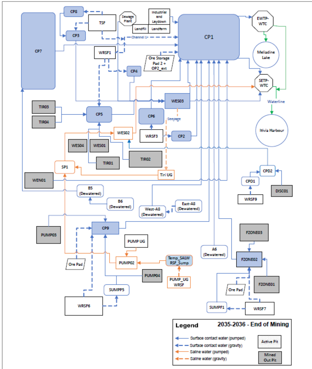
Figure 7: Conceptual Site Water Management Flow Diagram as Planned at the End of the Life of Mine
