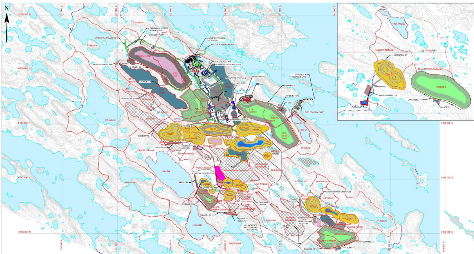
Figure 5: Mine Site Layout at 2036
