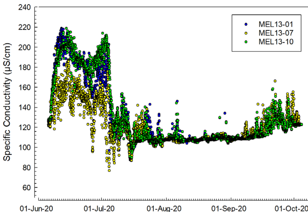
Figure B-6: Continuous Specific Conductivity Measurements at the Edge of Mixing Zone Stations Collected 2 m above the Lakebed from 5 June 2020 to 4 October 2020
