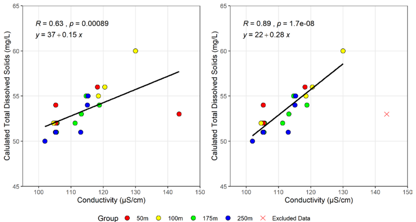
Figure 3: Linear Relationship Between Calculated Total Dissolved Solids and Conductivity at Meliadine Lake with (Left) and Without (Right) Extreme Conductivity Result
