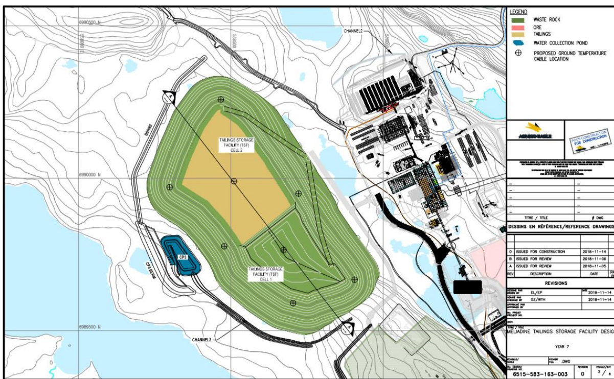
Figure 5.1 Tailings Placement Plan in Cells – Year 7
