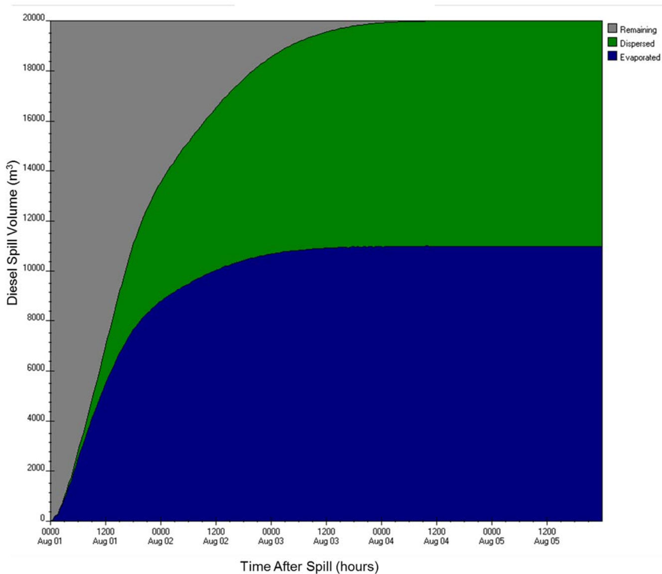
Figure E-A8: ADIOS2 diesel fuel budget output for two fuel transfer stations (1 and 2) near Melvin Bay for 20,000 m³, 2-yr wind speed scenario
