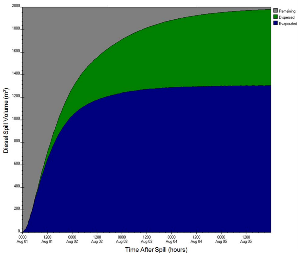
Figure E-A43: ADIOS2 diesel fuel budget output for Entrance to Melvin Bay station (3A) for 2,000 m 3 , mean wind speed scenario
