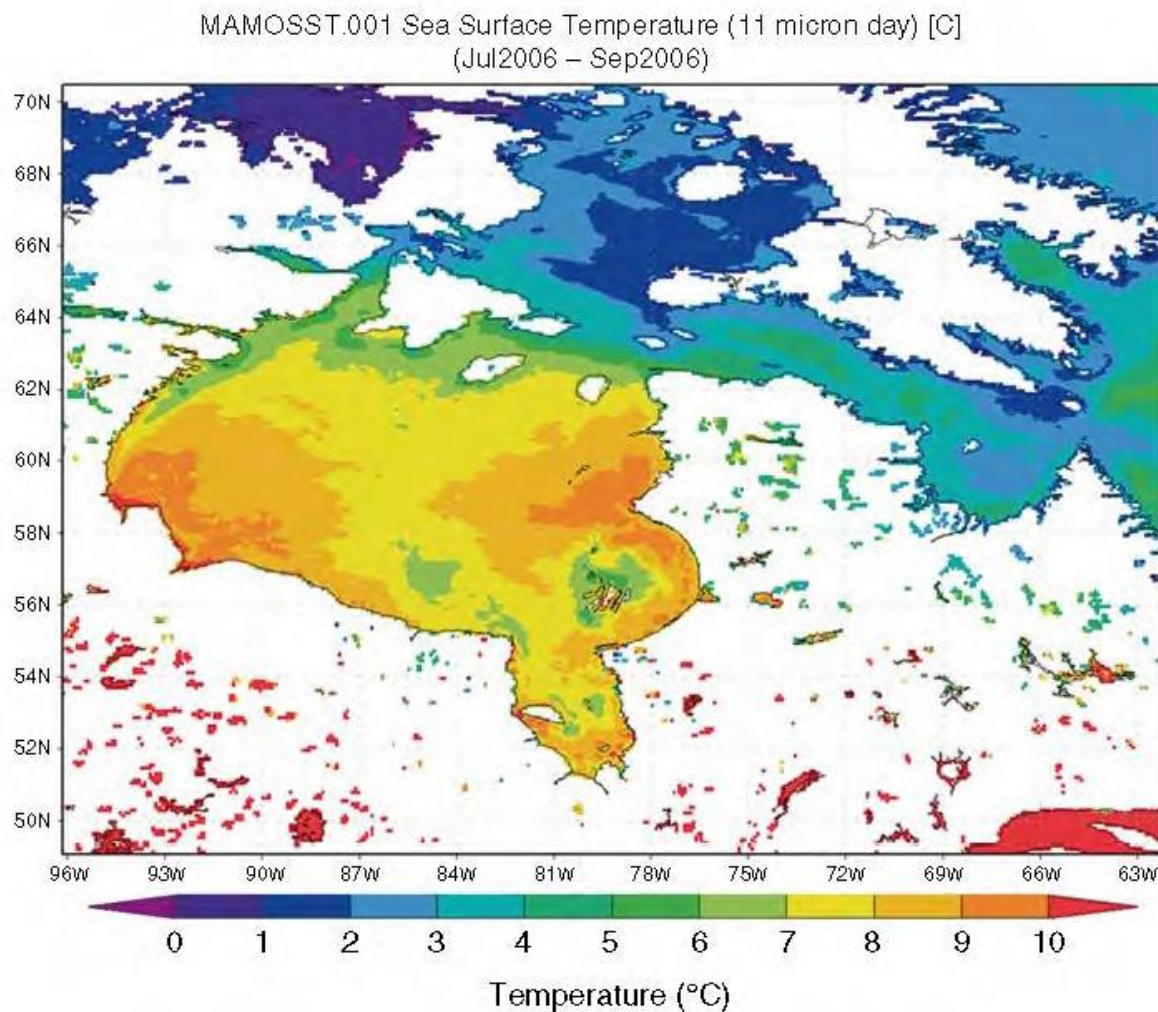
Figure B-6: Summer (July to September) sea surface temperature in 2006 (Stewart and Barber 2010)
