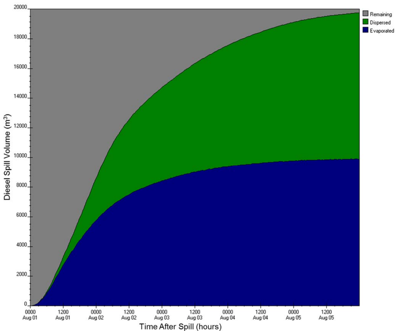
Figure E-A13: ADIOS2 diesel fuel budget output for Walrus Island station (3) for 20,000 m³, mean wind speed scenario
