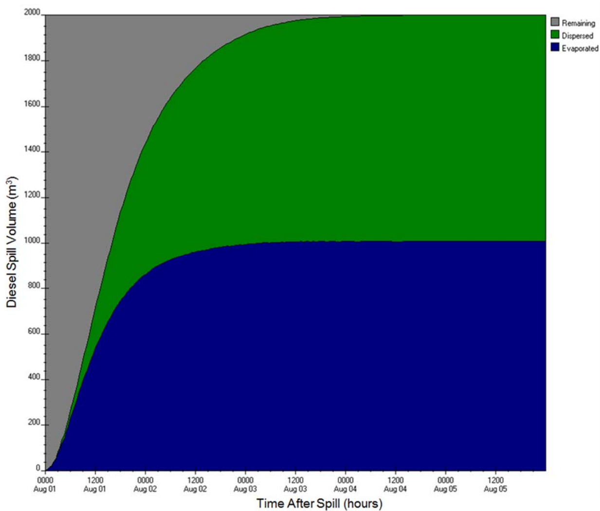
Figure E-A72: ADIOS2 diesel fuel budget output for Eastern Hudson Strait station (8A) for 2,000 m³, mean wind speed scenario
