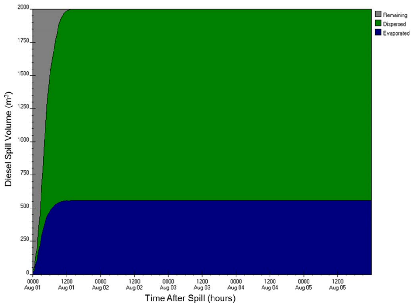
Figure E-A11: ADIOS2 diesel fuel budget output for Walrus Island station (3) for 2,000 m 3 , 2-yr wind speed scenario
