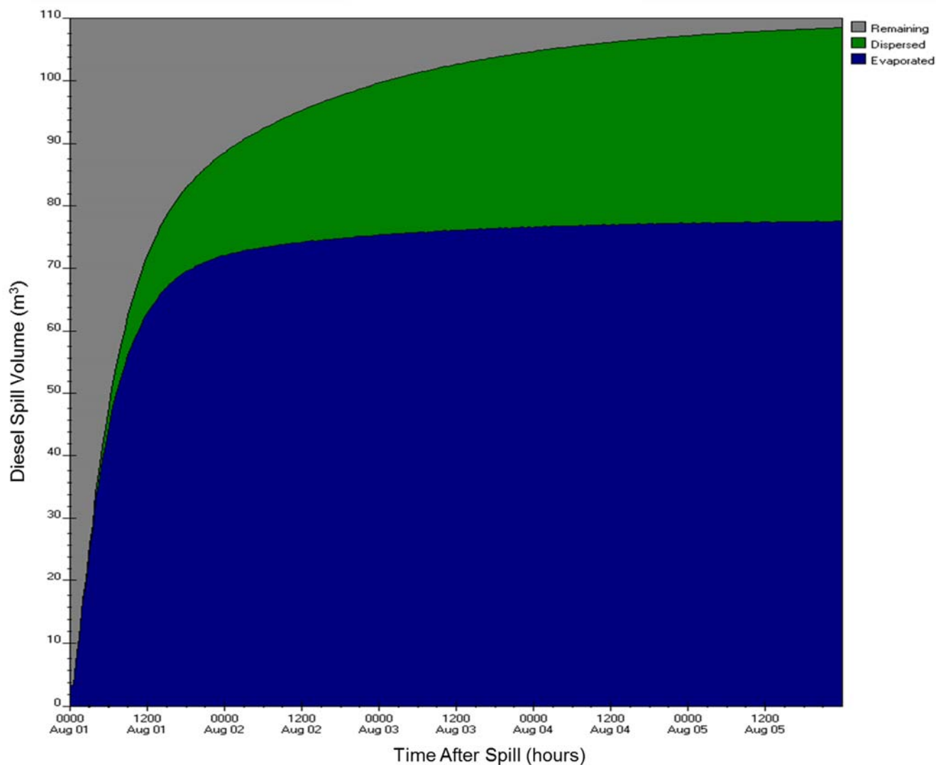
Figure E-A1: ADIOS2 diesel fuel budget output for two fuel transfer stations (1 and 2) near Melvin Bay for 100 m 3 , mean wind speed scenario
