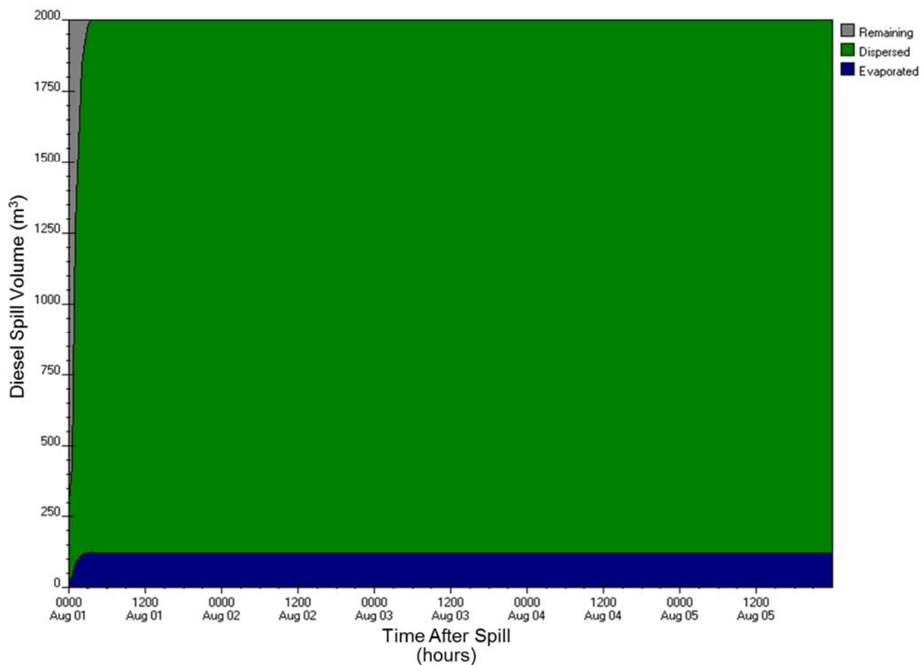
Figure E-A30: ADIOS2 diesel fuel budget output for Eastern Hudson Strait station (6) for 2,000 m³, 50-yr wind speed scenario
