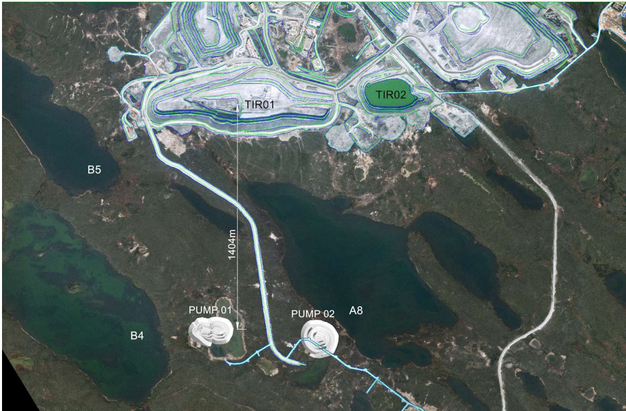
Figure 10 - Open Pit Surface Plan – Pump (Final Pit Shell)
