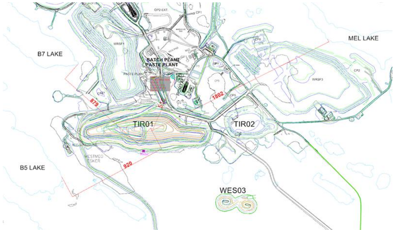
Figure 4. Surface blast monitoring station locations for TIR01 blasts (distances in meters)
