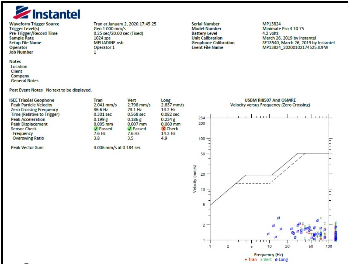
Figure 8. InstanTEL Sample Vibration Report
