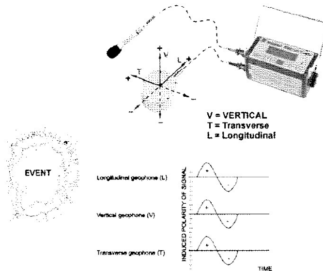
Figure 2. Sensor Orientation
