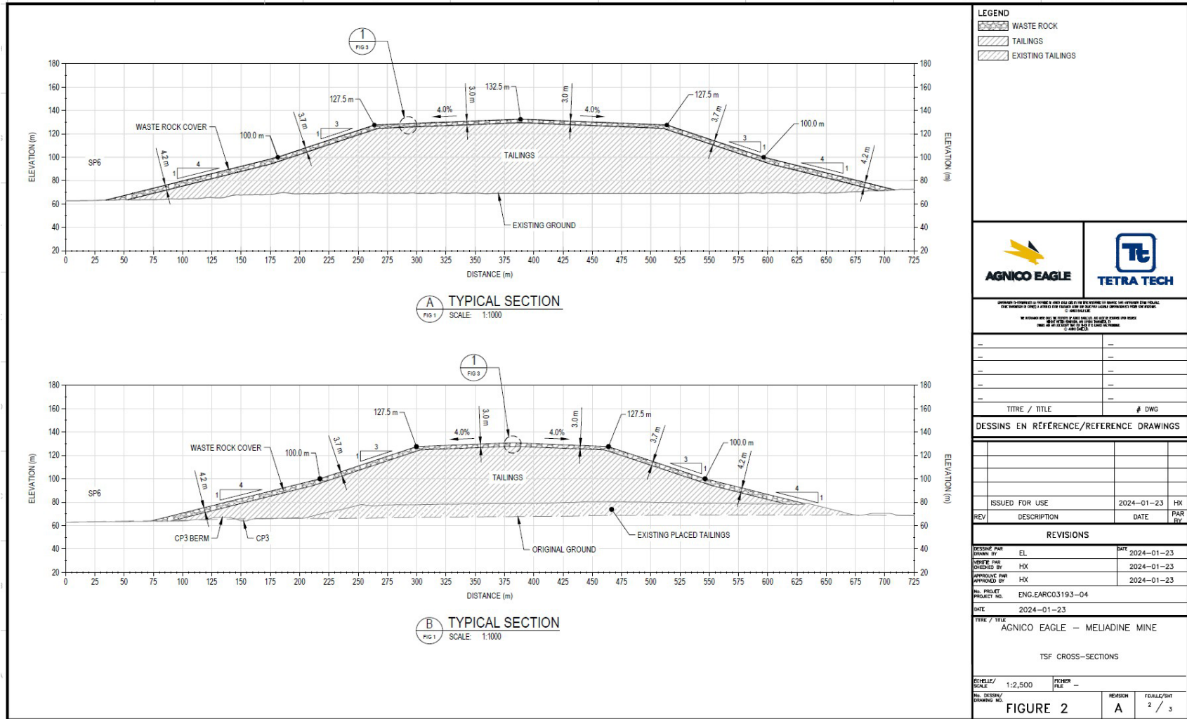
Figure 4.1: Typical Design Cross-Section for TSF
