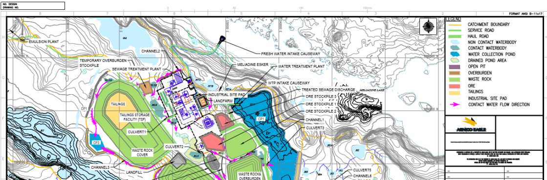
Figure 6.1 Mine Site Layout for Water Management During Closure from Feasibility Level Study. (TetraTech, 2014).
