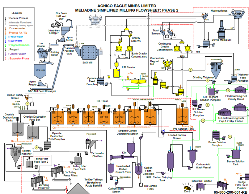
Figure 4-5 : Meliadine Mineral Processing Flowsheet
