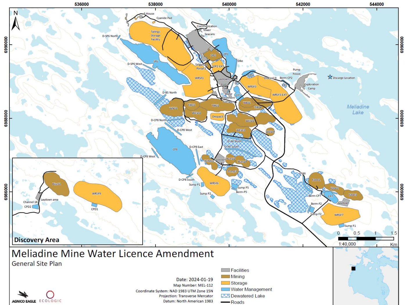
Figure 2 General Mine Site Plan Layout
