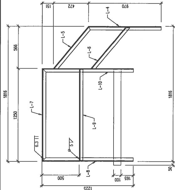
1L/1R REQ'D REMOVABLE HANDRAIL ARRANGEMENT
