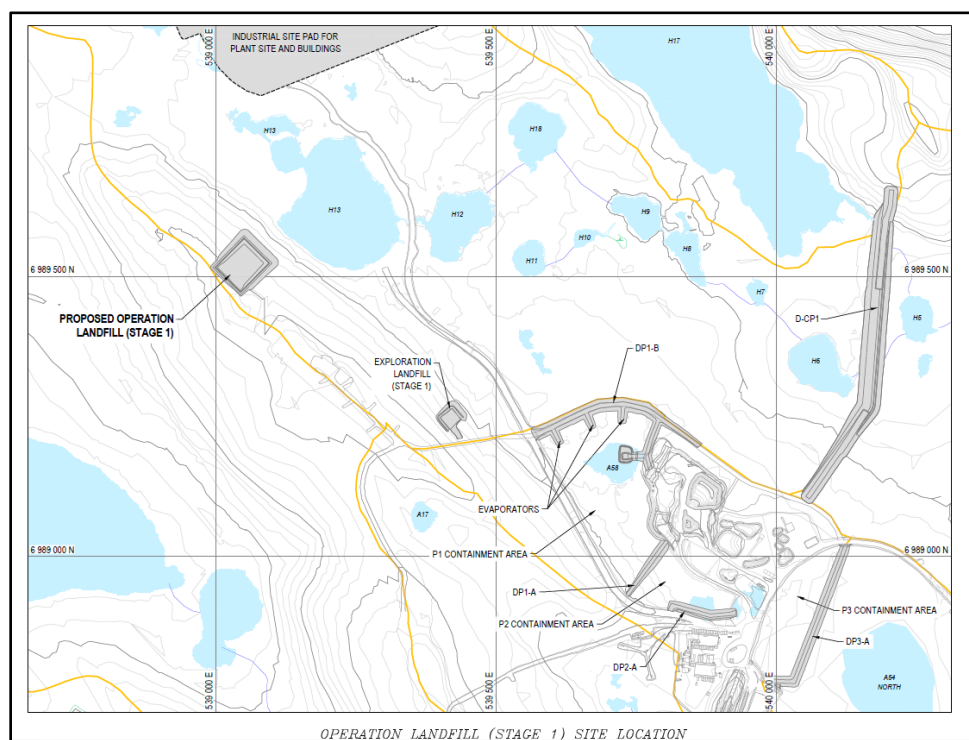
Figure 5-5 : Operation Landfill (Stage 1) Location
