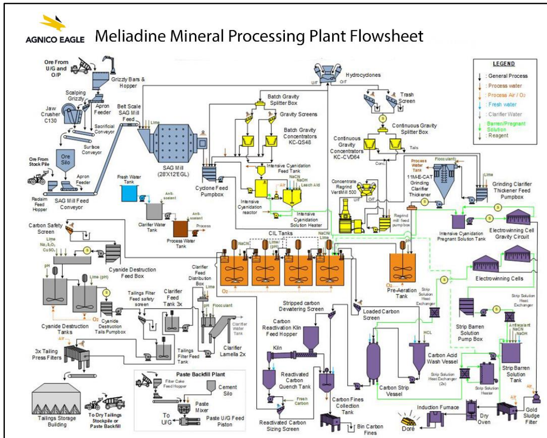
Figure 5-4 : Meliadine mineral processing flowsheet
