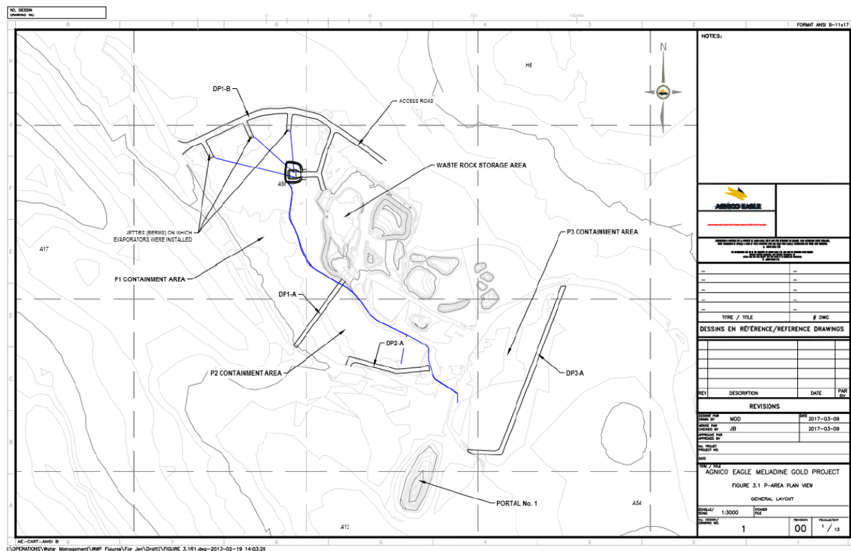
Figure 5-3 : P-Area plan view and general location
