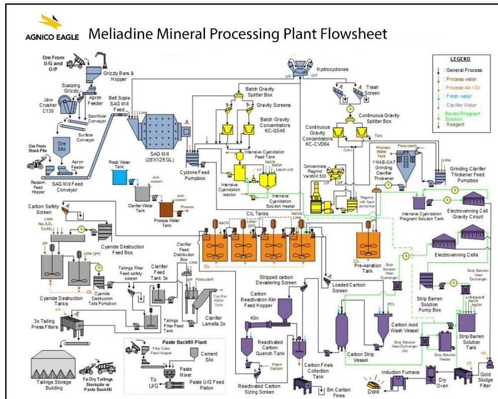
Figure 5-6 : Meliadine mineral processing flowsheet
