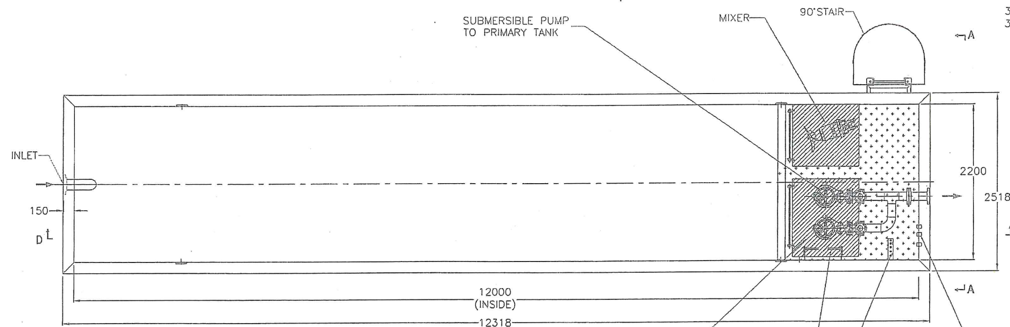
PLAN VIEW
