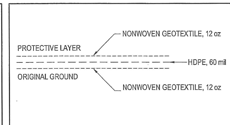
LINER DETAIL
