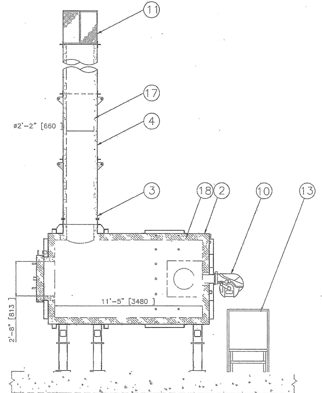
SECTION C-C
