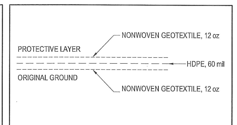
LINER DETAIL
