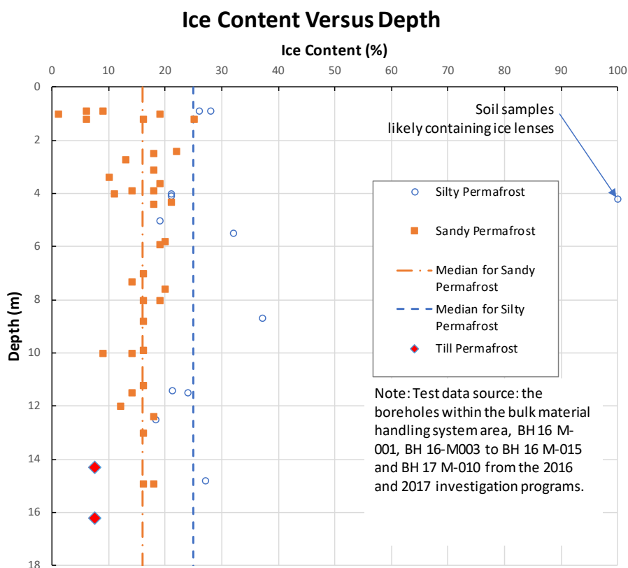
Figure 3-1: Ice Content in Permafrost with Depth
