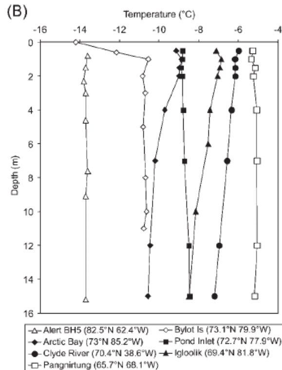
Figure 3-5: Mean annual ground temperature profiles during the International Polar Year for selected sites in the eastern and high Canadian Arctic (Smith et. al. 2010)
