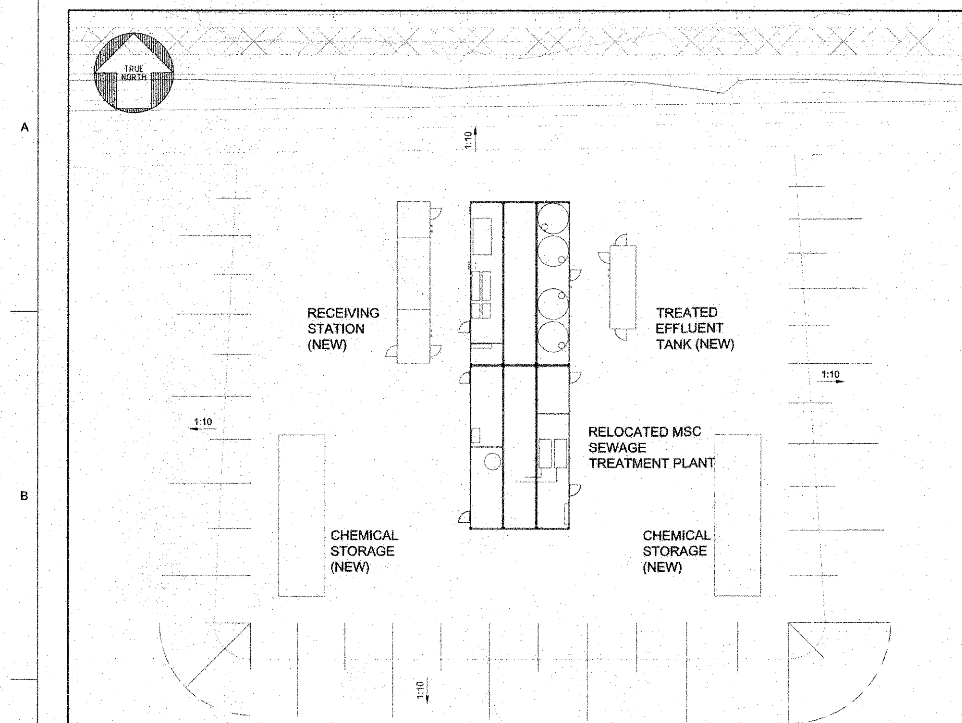
ENLARGED DETAIL OF SEWAGE TREATMENT PLANT #2 SCALE 1:250
