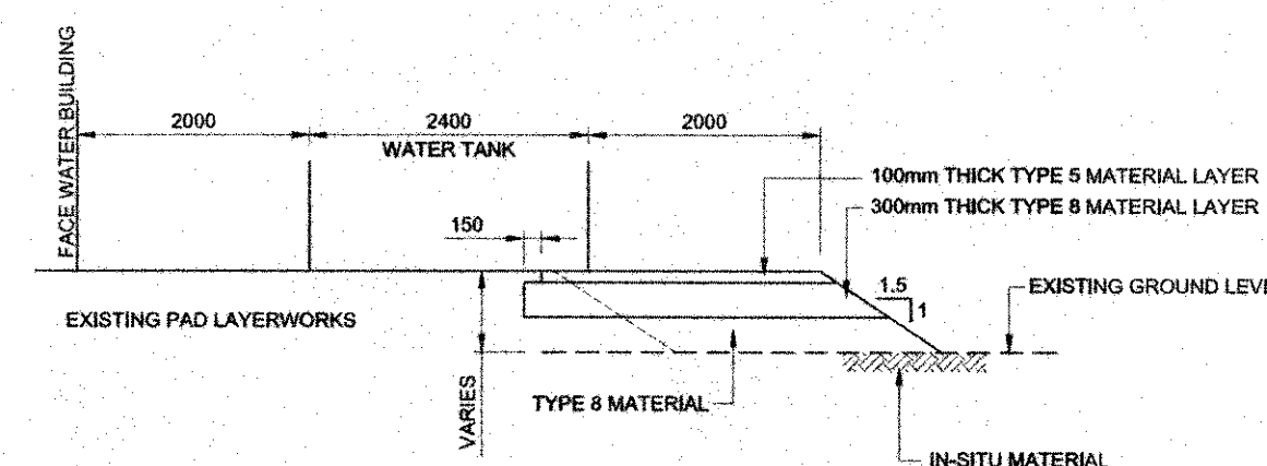
TYPICAL SECTION - WATER TANK PAD SCALE 1:50 THIS SECTIONAL DETAIL IS TO BE READ IN CONJUNCTION WITH DWG. No. H353004-00000-221-294-0003-0001.
