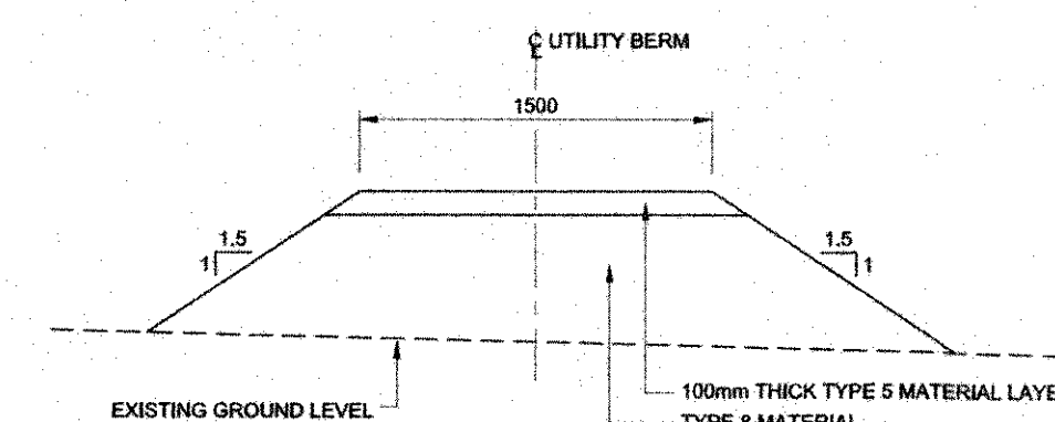
TYPICAL SECTION - UTILITY BERM SCALE 1:25 THIS SECTIONAL DETAIL IS TO BE READ IN CONJUNCTION WITH DWG. No. H353004-00000-221-294-0003-0001.
