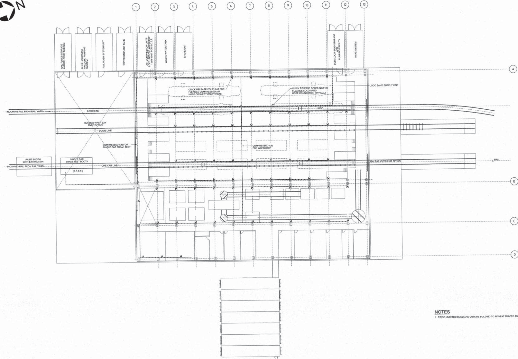
RAIL WORKSHOP FLOOR PLAN
