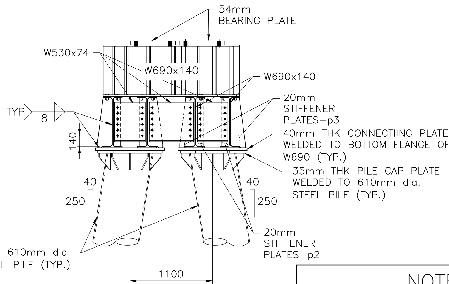
SECTION "C-C"
