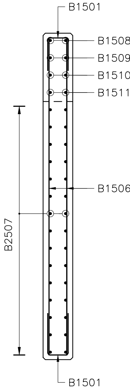
SECTION "C-C"
