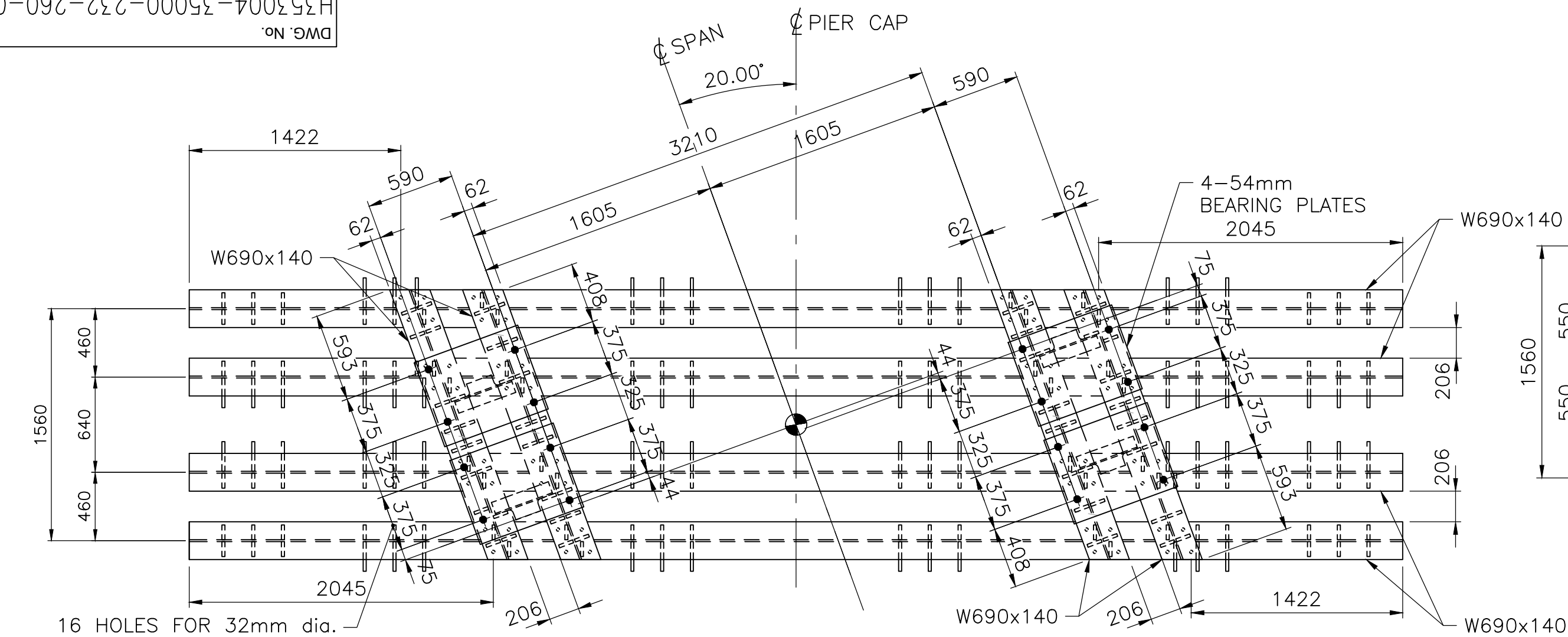
VIEW "A-A"
