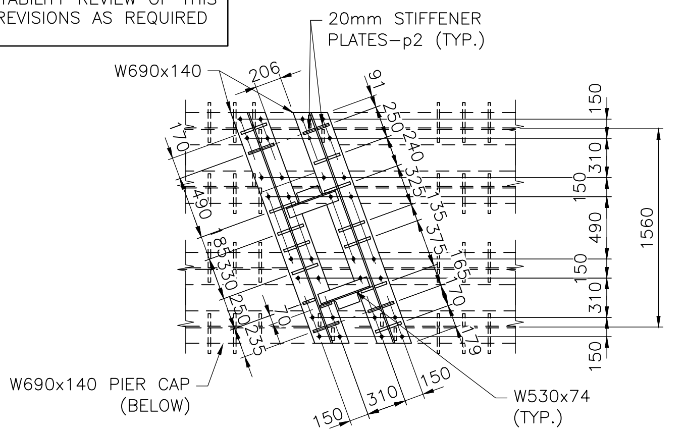
SECTION "G-G"
