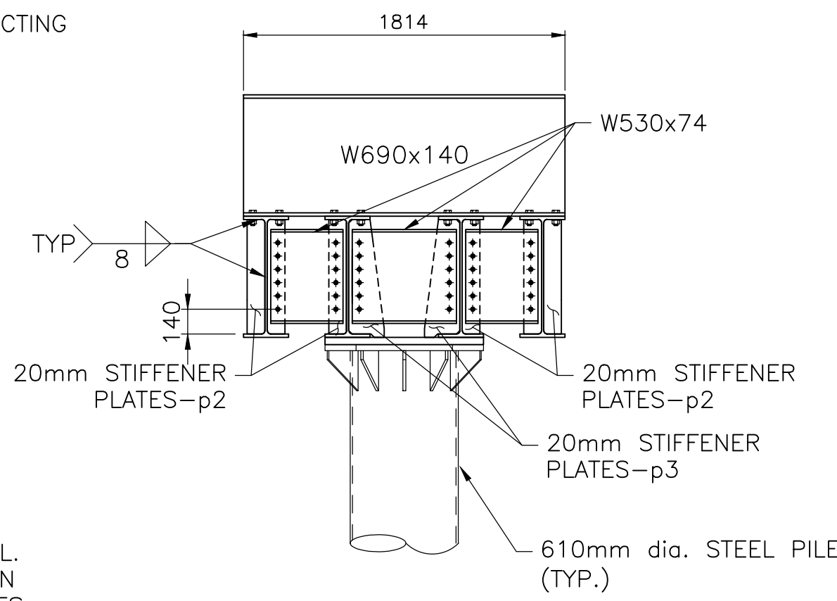
SECTION "E-E"
