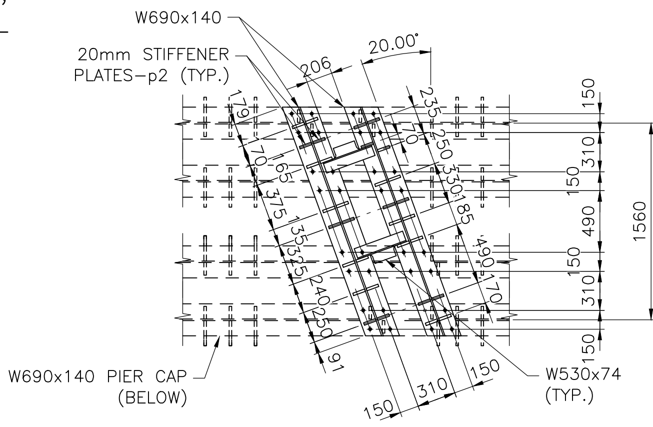
SECTION "F-F"
