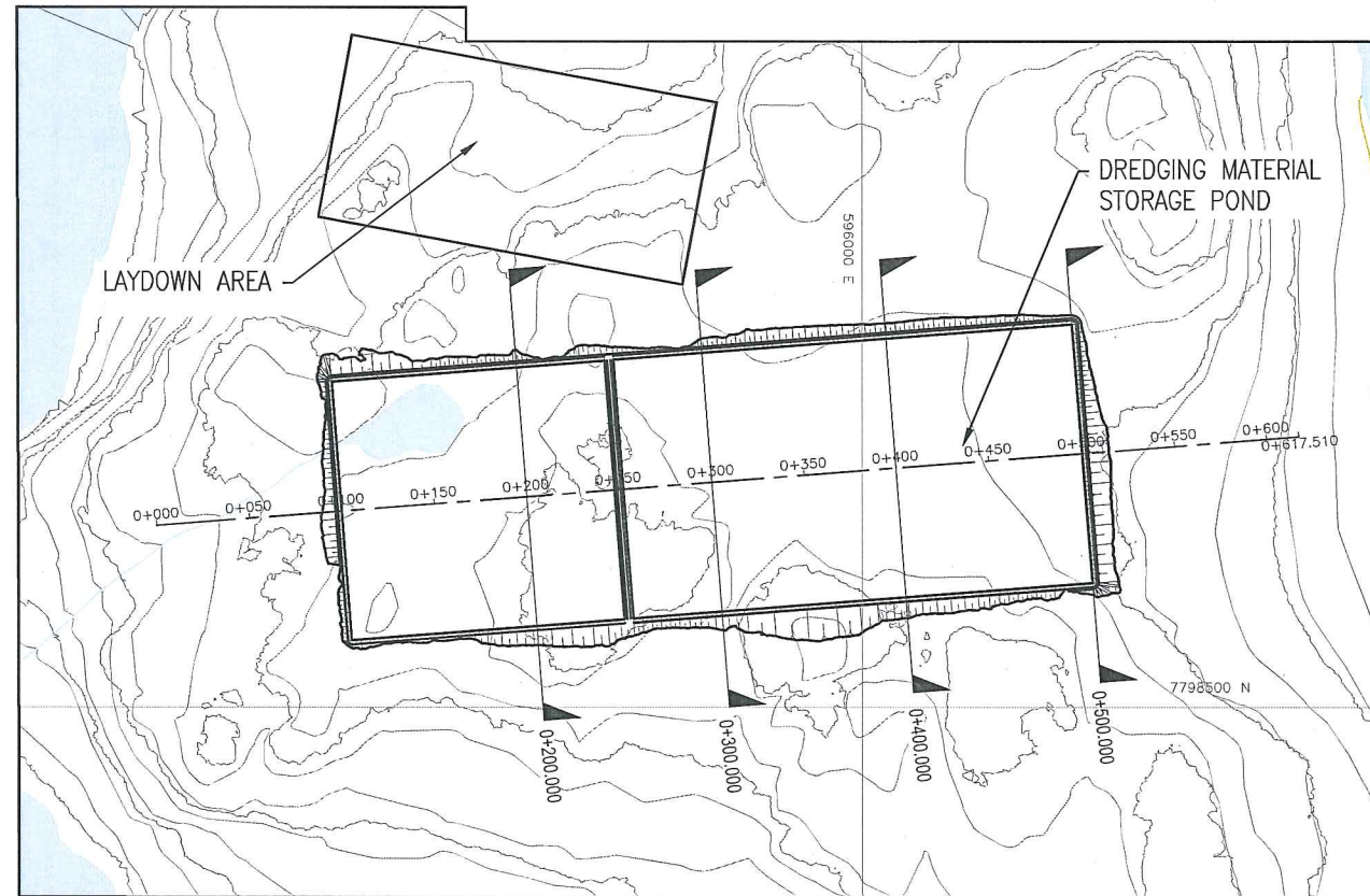
DREDGING INFILL PLAN
