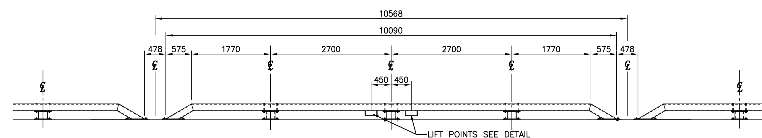
REMOVABLE WHEEL GUARD
