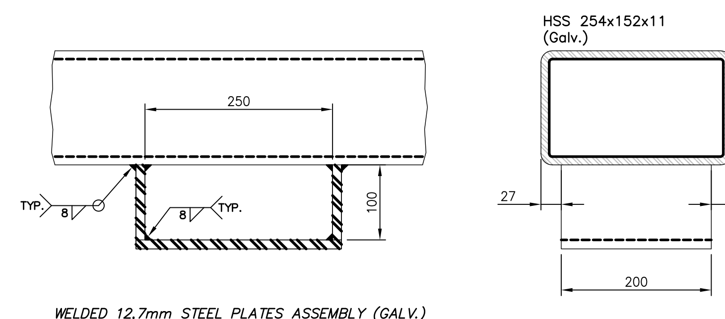
LIFT POINT DETAIL SCALE: 1:5
