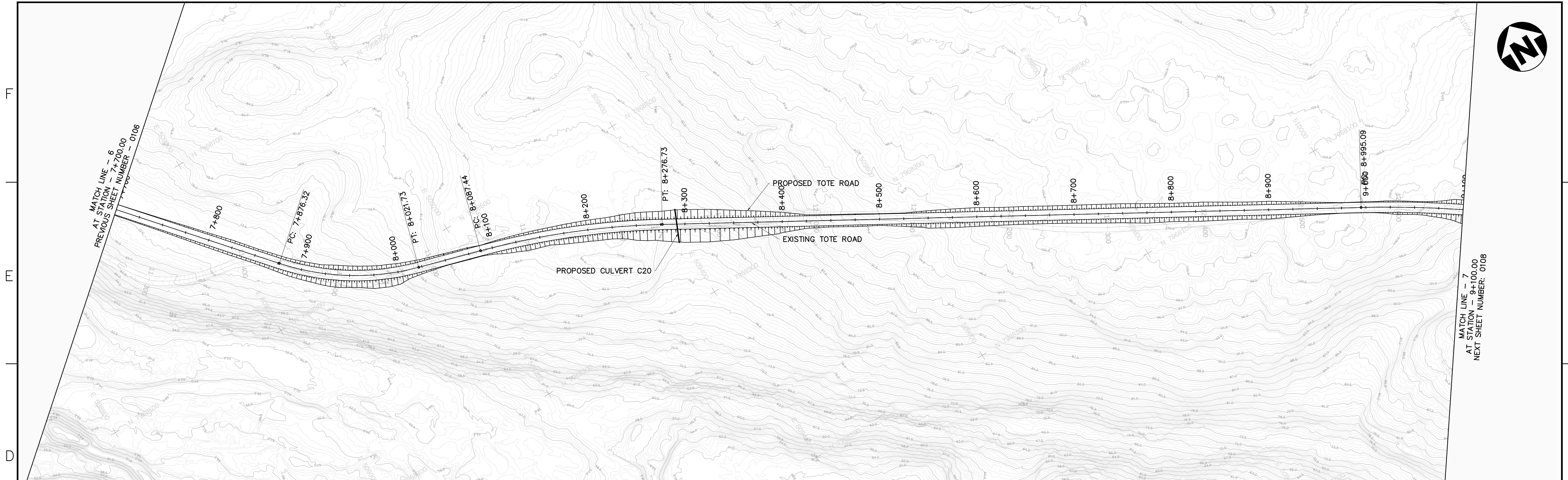
TOTE ROAD PLAN
