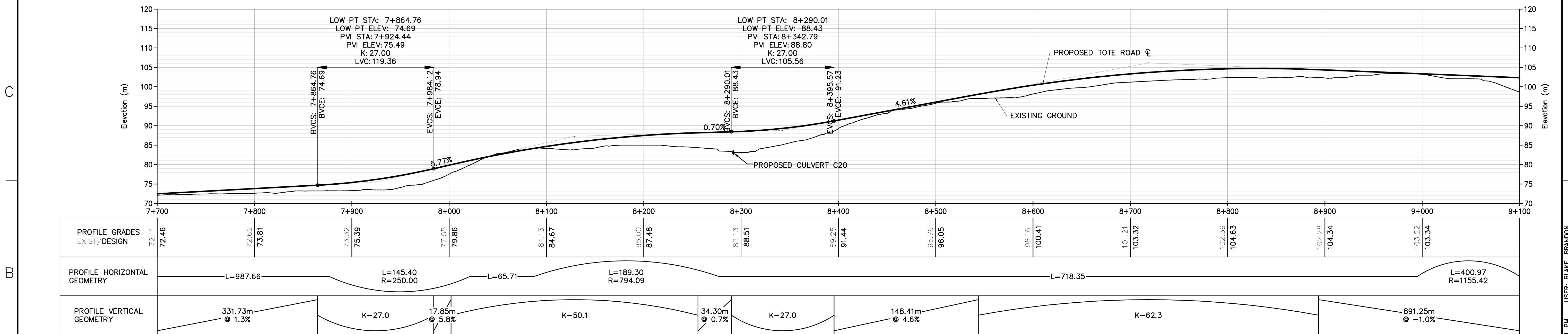
TOTE ROAD PROFILE
