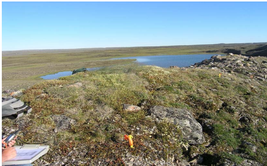
Photo 121. Crest of esker, enriched due to animal use, Plot 06_VN016.
