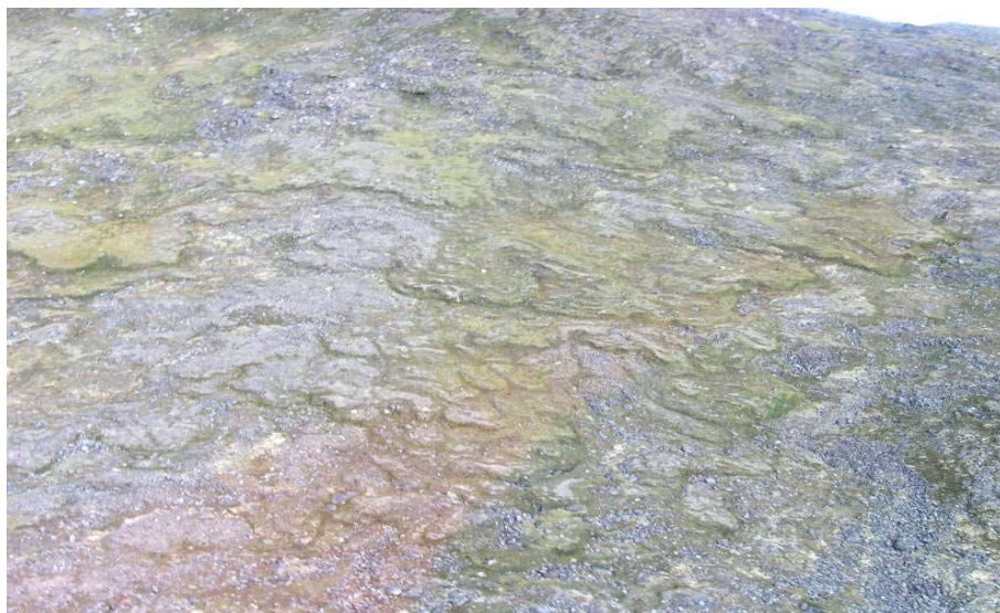
Photo 143. Solifluction slope from air.
