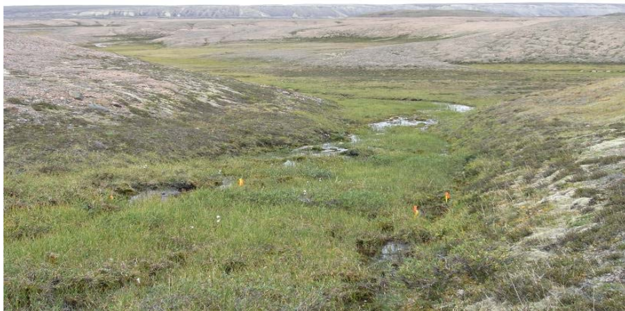
Photo 129. Glaciofluvial complex, sedge association in valley in complex, Plot 06_VN343.
