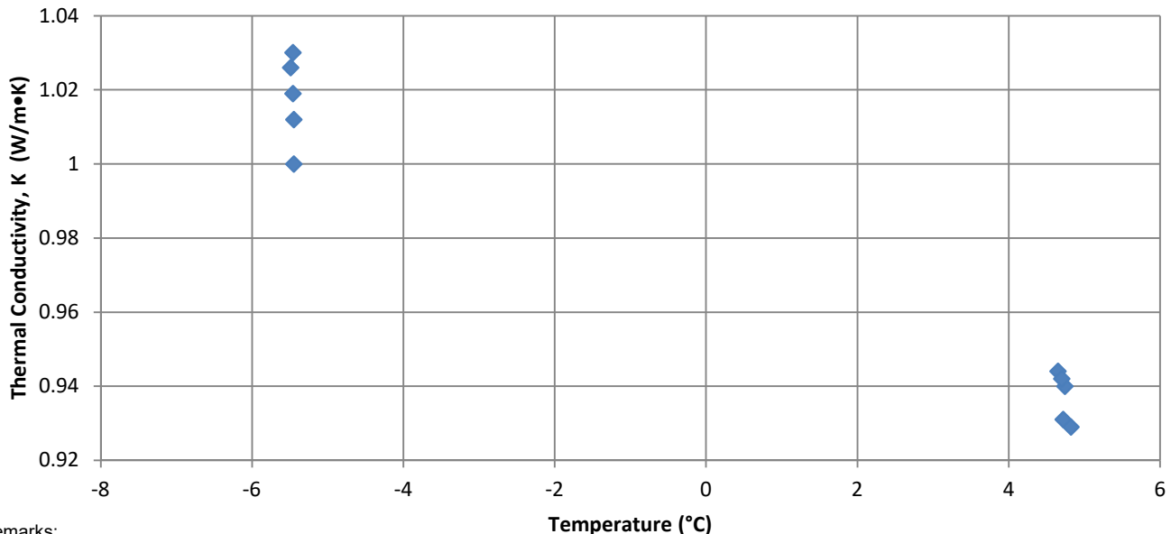
Thermal Conductivity vs. Temperature
