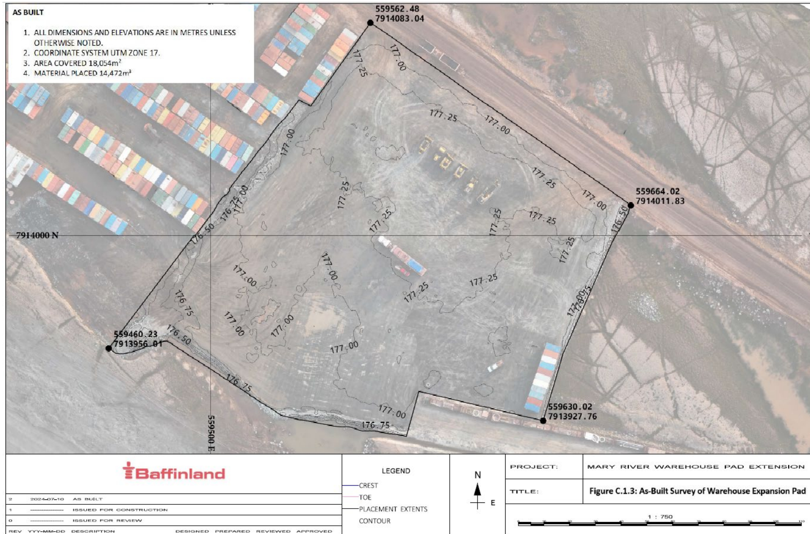
Figure C.1.3: As-Built Survey of Warehouse Expansion Pad
