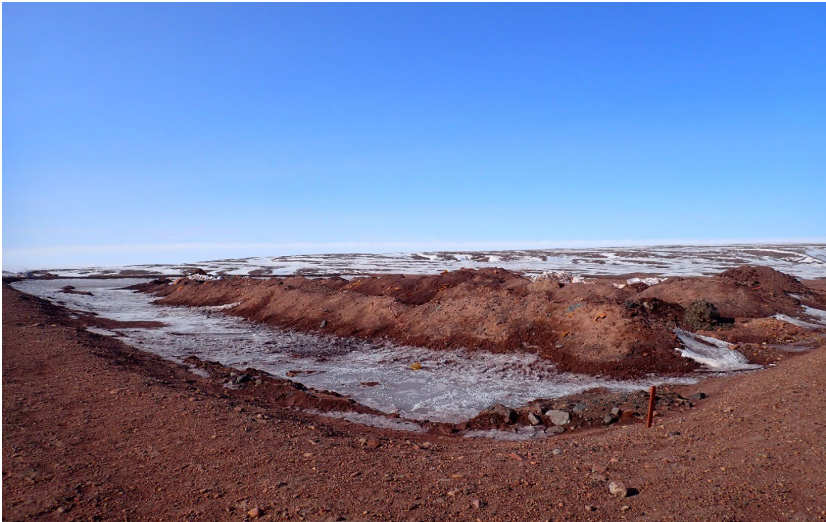
Photo 45. Soil Windrows in the Landfarm Facility Cell 1 - May
