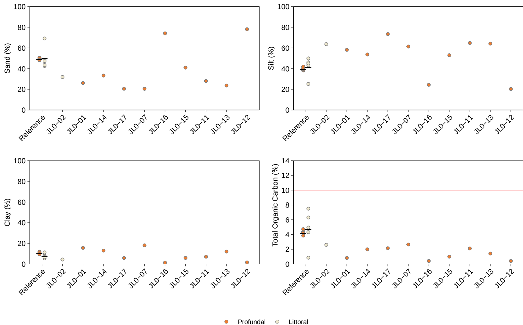
Figure 3.8: Sediment Particle Size and Total Organic Carbon (TOC) Content Comparisons among Core Samples taken from Camp Lake (JLO) Sediment Monitoring Stations and Reference Lake 3 (REF-03), Mary River Project CREMP, August 2024
