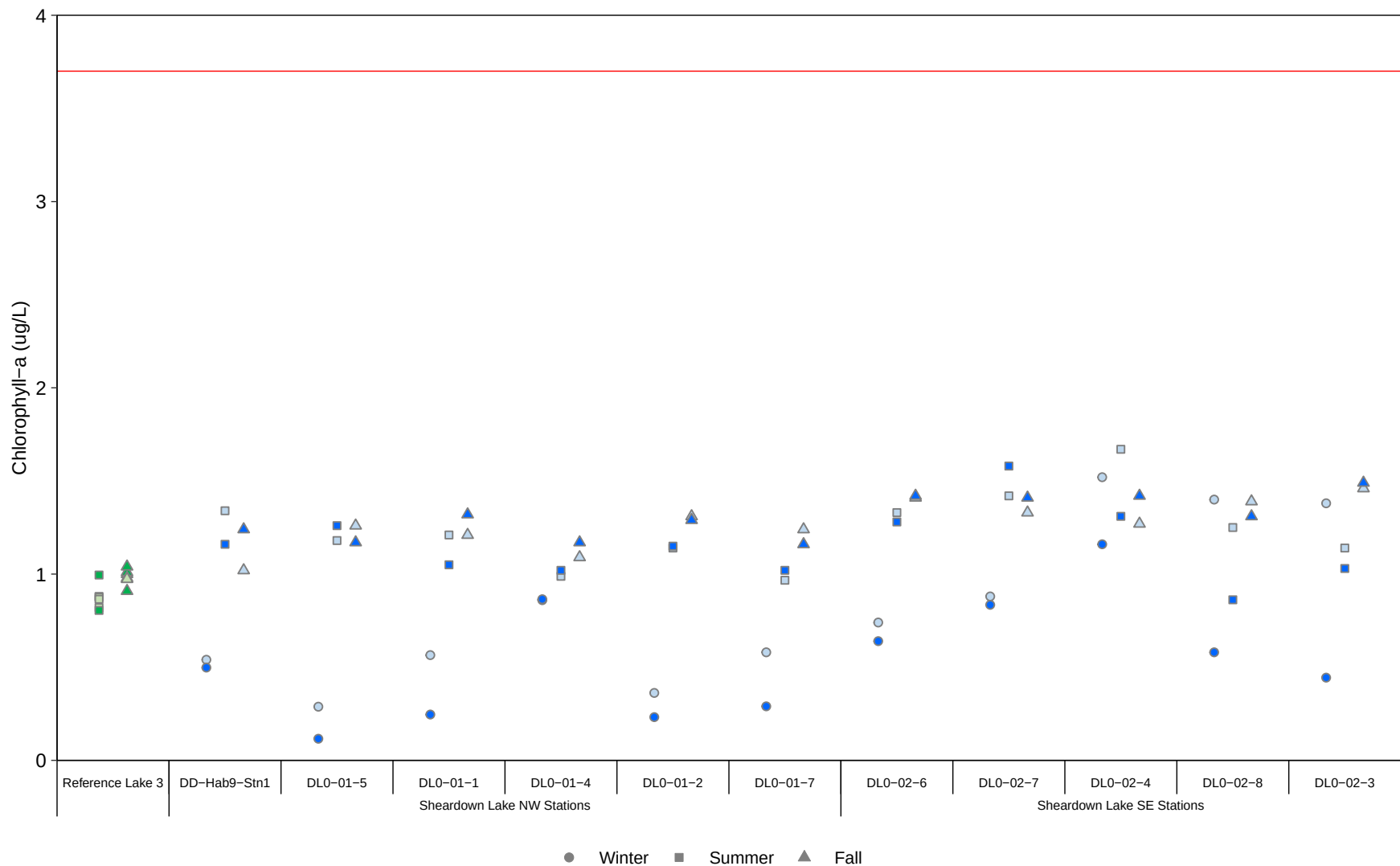
Figure 4.8: Chlorophyll-a Concentrations at Sheardown Lake Northwest (NW; DL0-01) and Sheardown Lake Southeast (SE; DL0-02) Phytoplankton Monitoring Stations, Mary River Project CREMP, 2024
