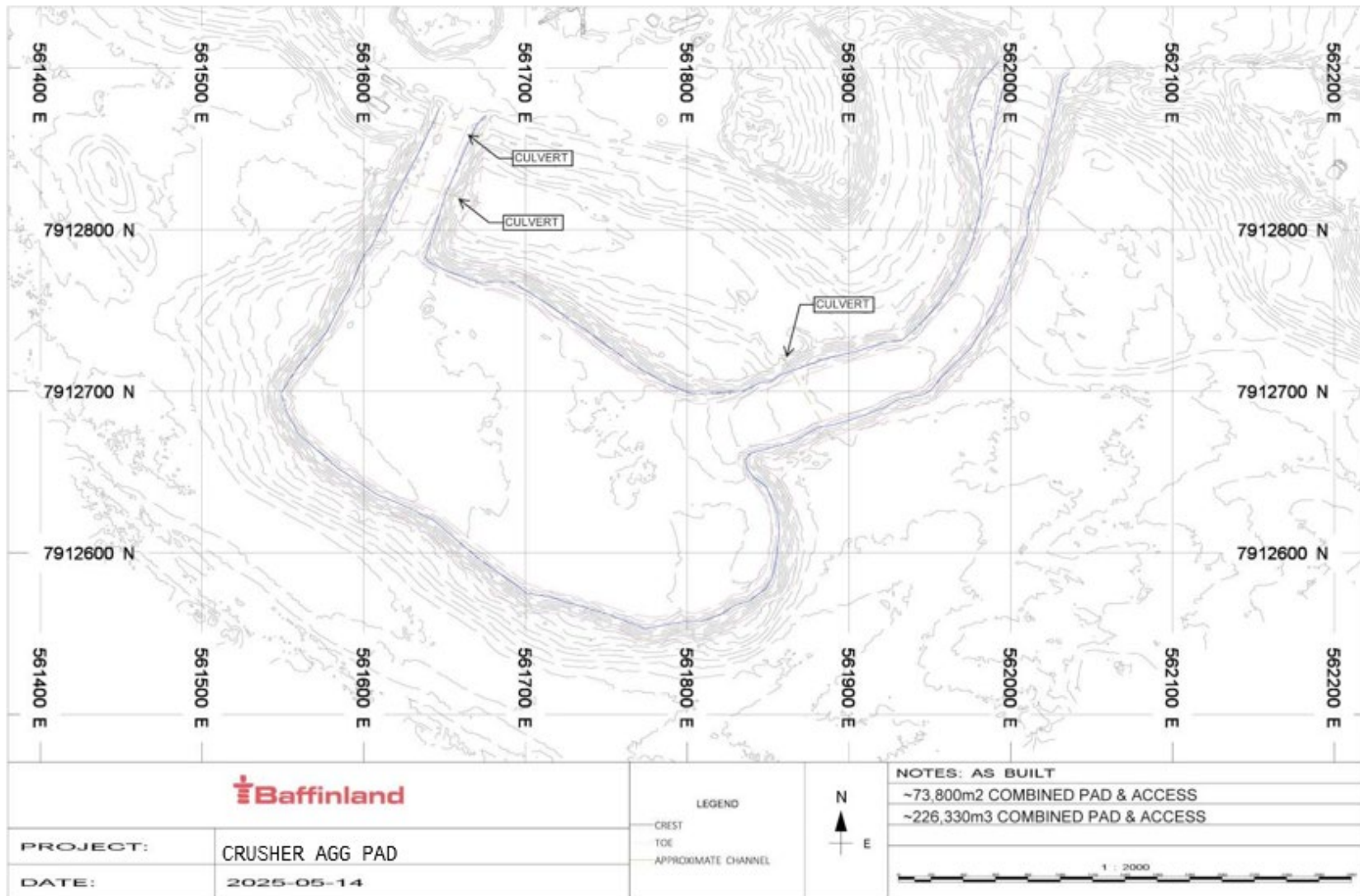
Figure C.1.1: As-Built Survey of Additional Crusher Pad
