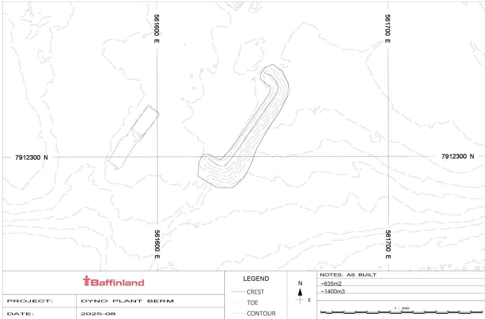
Figure C.1.3: As-Built Survey of Magazine Explosives Berm
