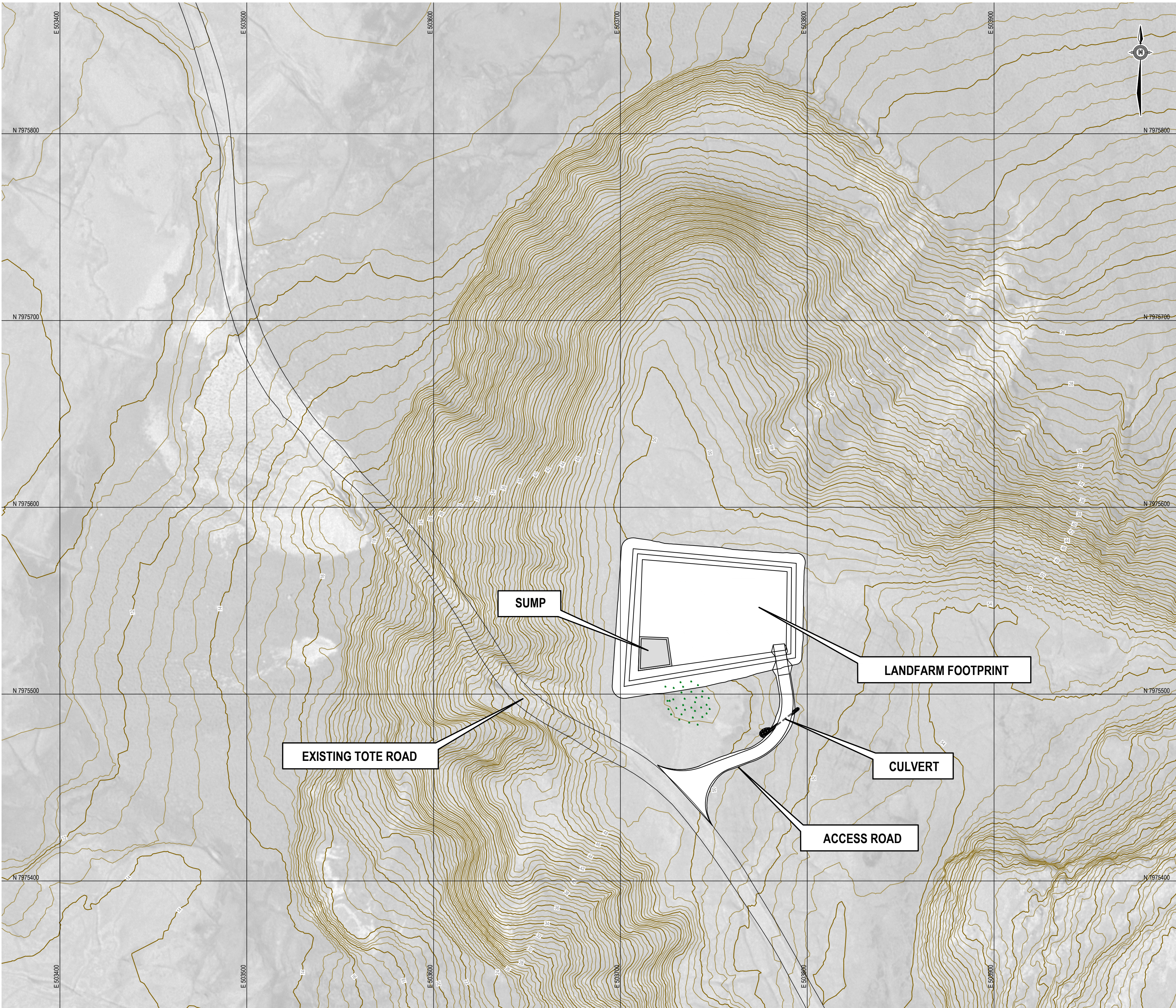
GENERAL SITE ARRANGEMENT
