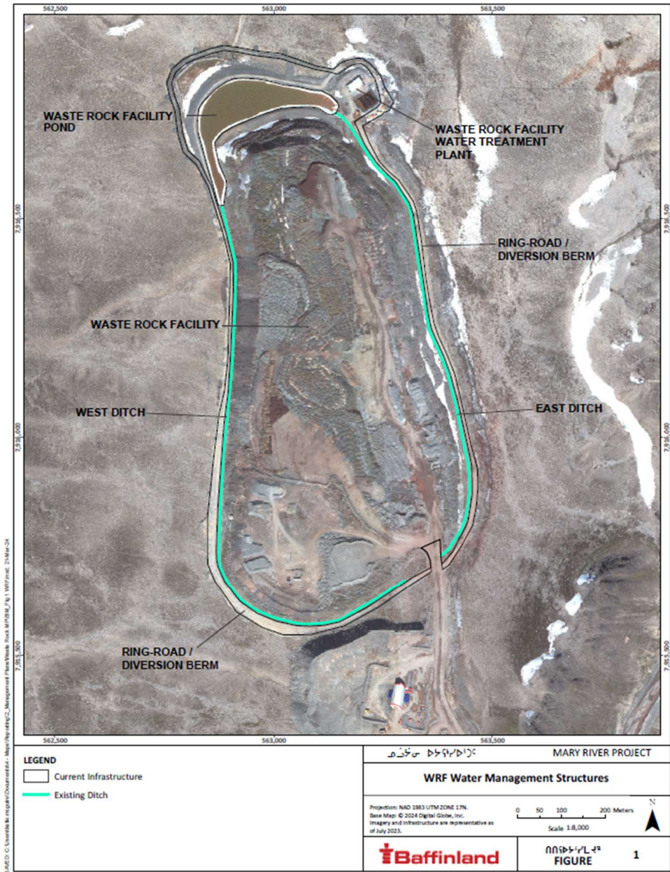
FIGURE 1: WRF WATER MANAGEMENT STRUCTURES
